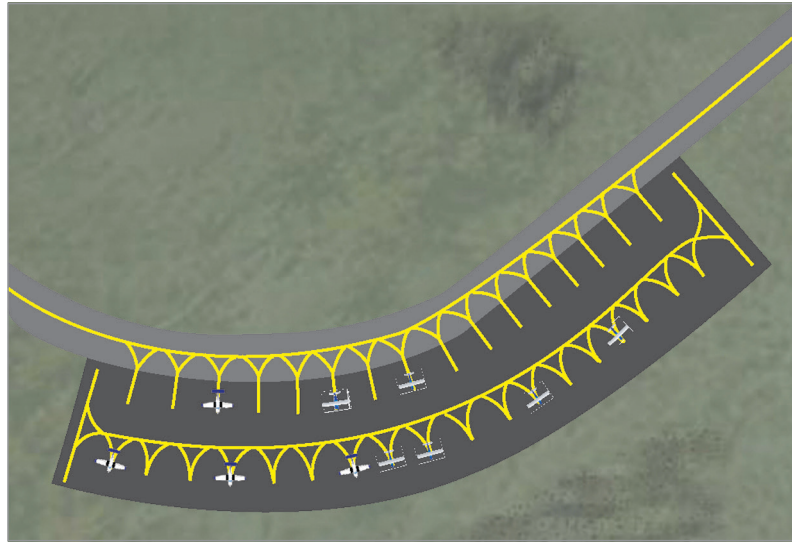
Figure 20.9 Example of aircraft stand markings
