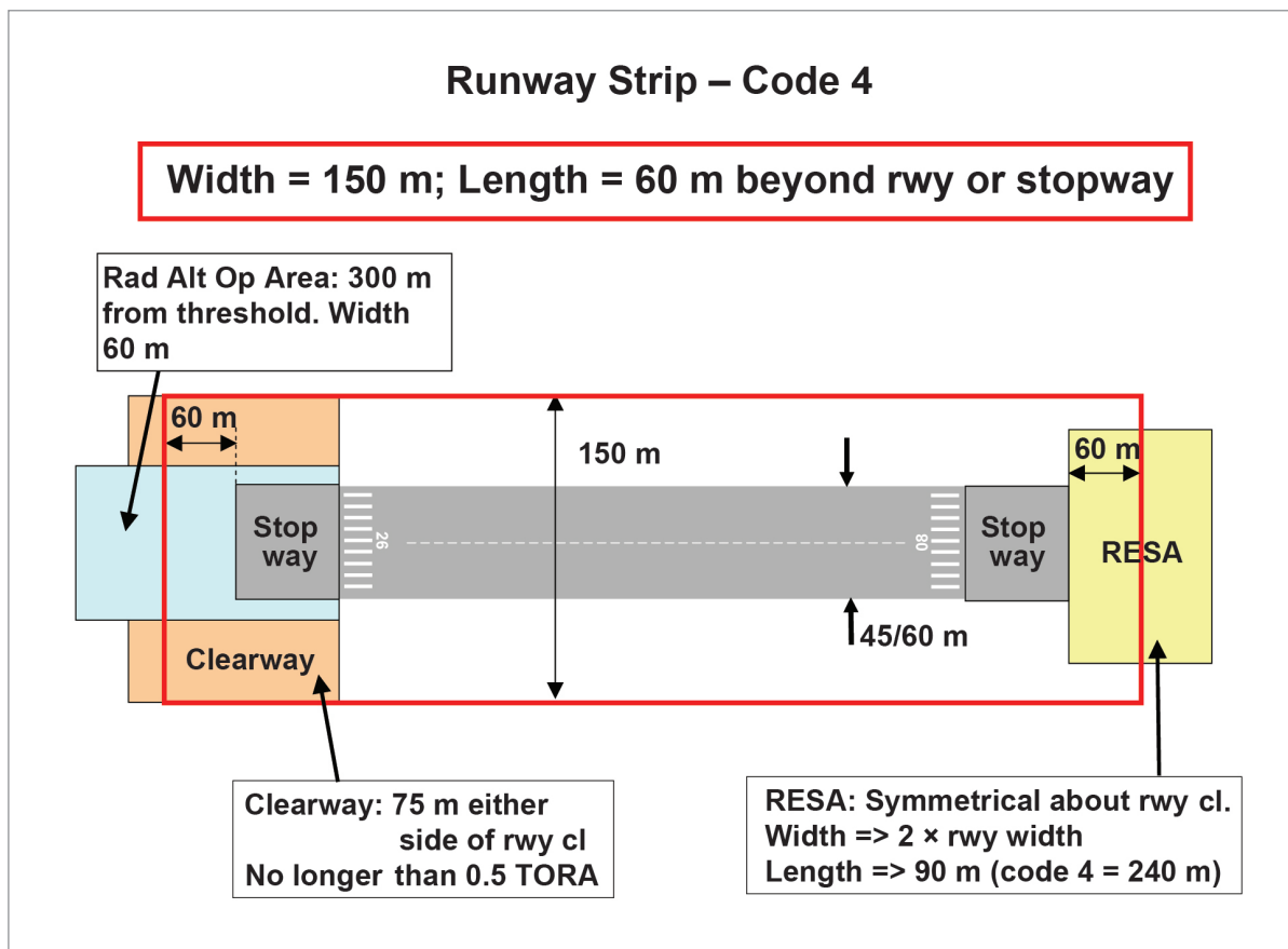
Figure 19.6 Runway strip - Code 4
