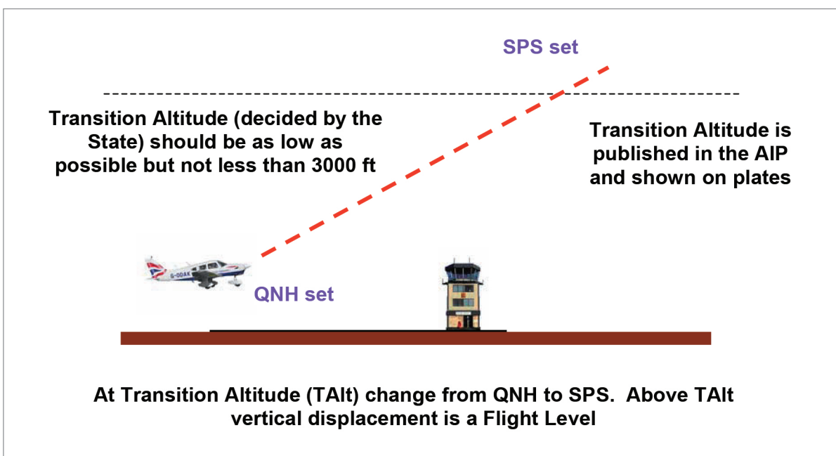
Figure 11.2 Transition altitude
