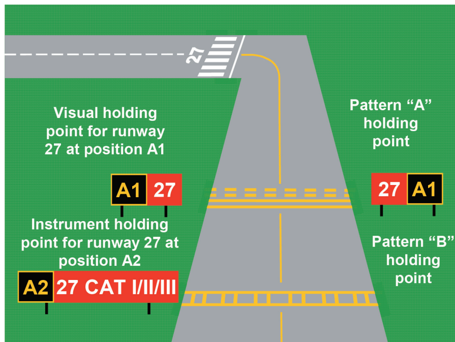
Figure 20.15 Information signs
