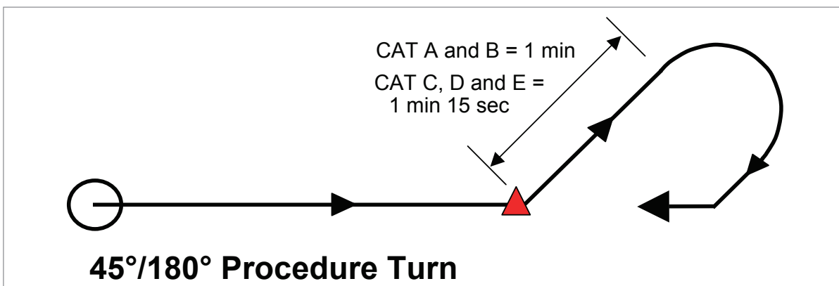
Figure 8.18 45°/180° - procedure turn
