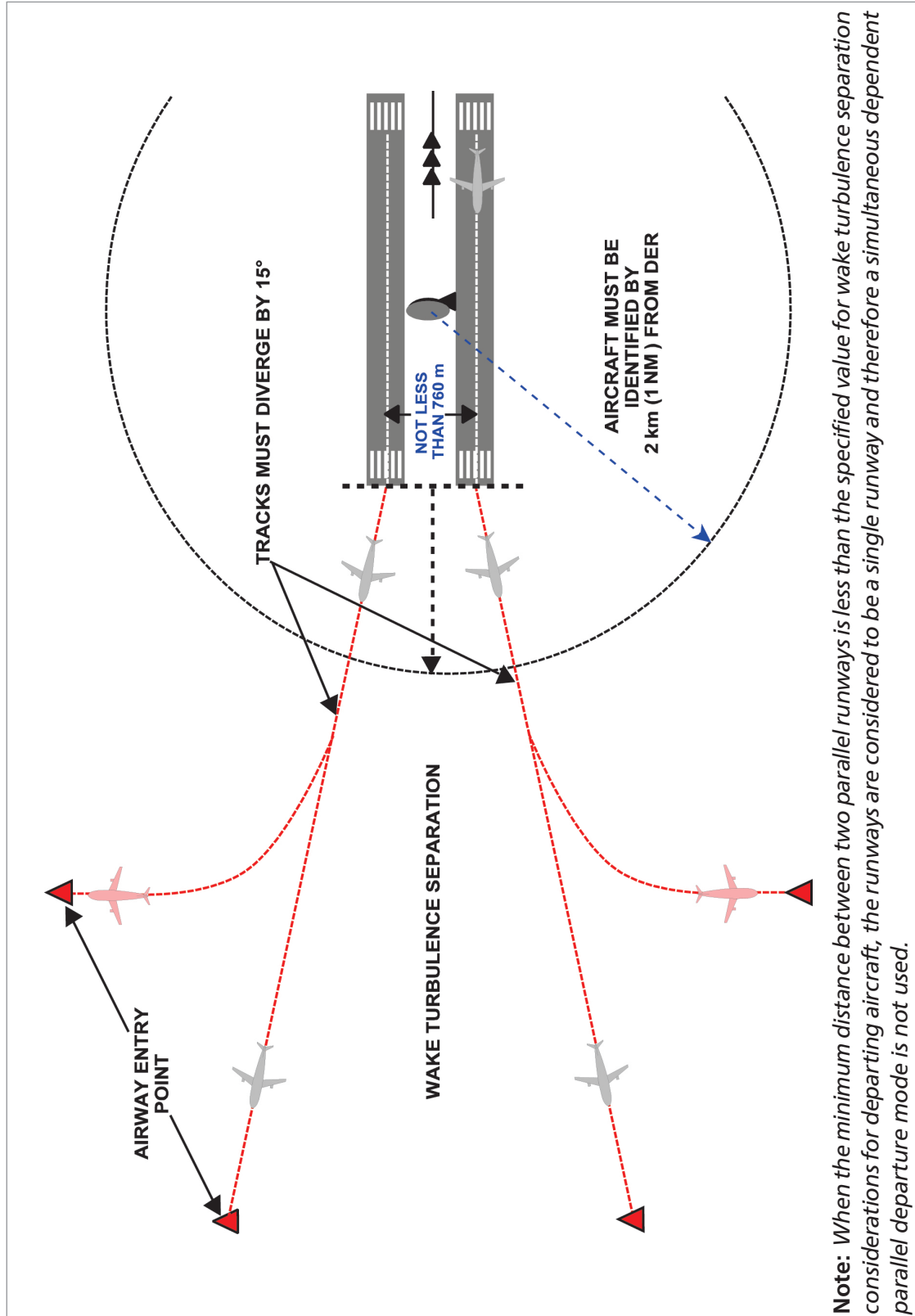
Figure 12.3 Mode 3 - Simultaneous instrument departures
