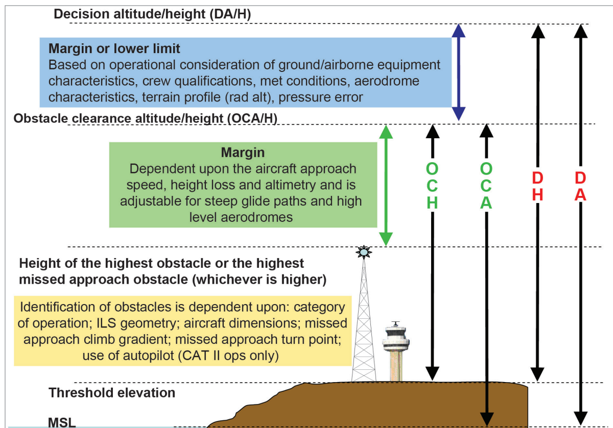
Figure 8.13 Method of determining DA/H for precision approaches
