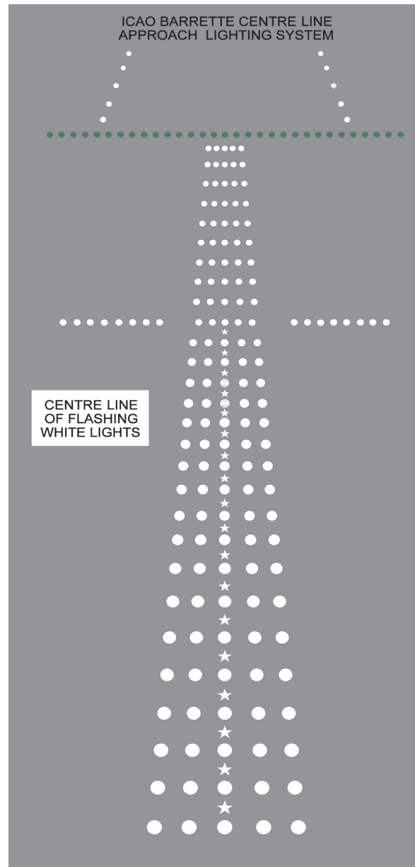
Figure 21.3 ICAO CAT I approach lighting system
