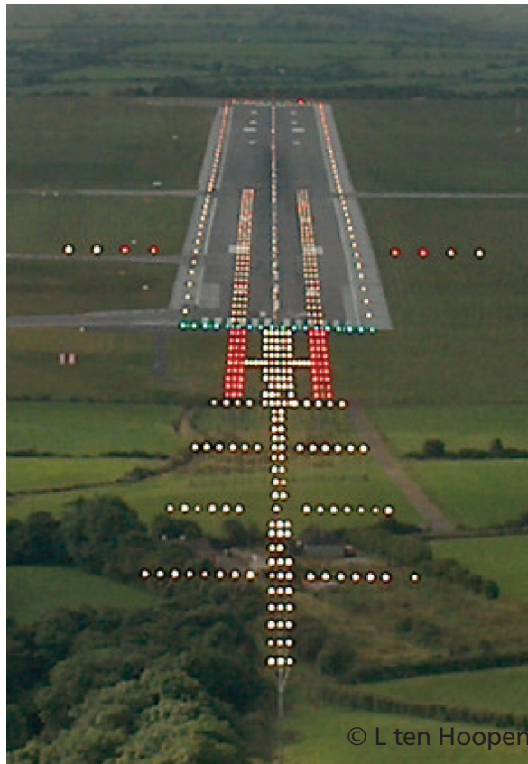
Figure 21.6 Calvert Cat II/III system at Cork
