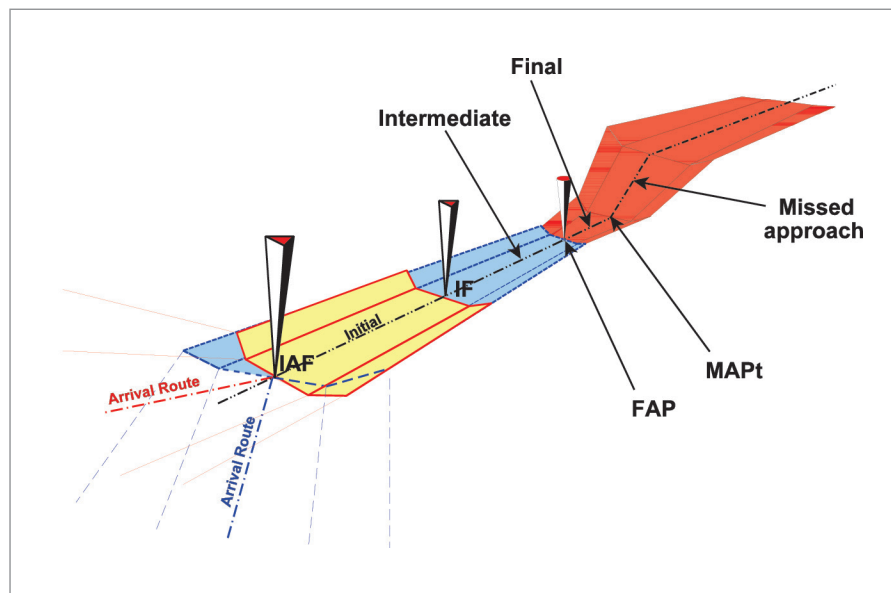
Figure 8.3 Procedure segments
