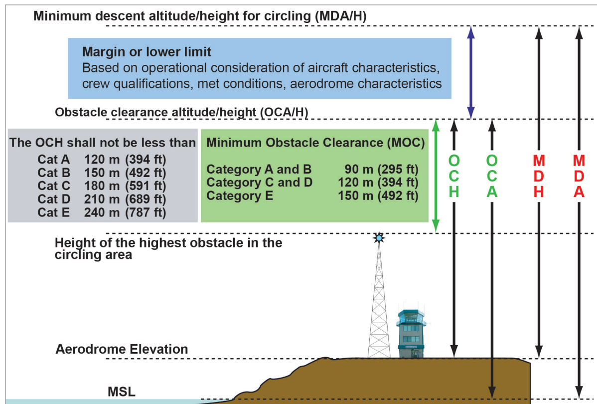
Figure 8.16 Method of determining MDA/MDH for circling approaches
