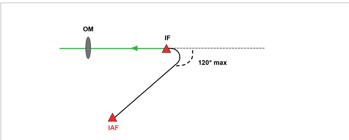
Figure 8.9 IAF to IF (non-precision approach)
