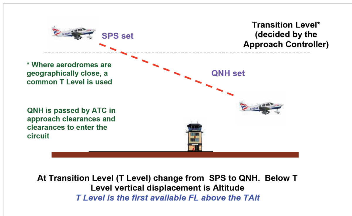
Figure 11.3 Transition level
