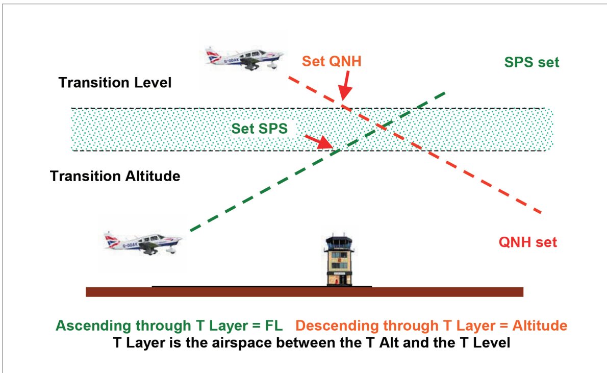
Figure 11.4 Transition layer
