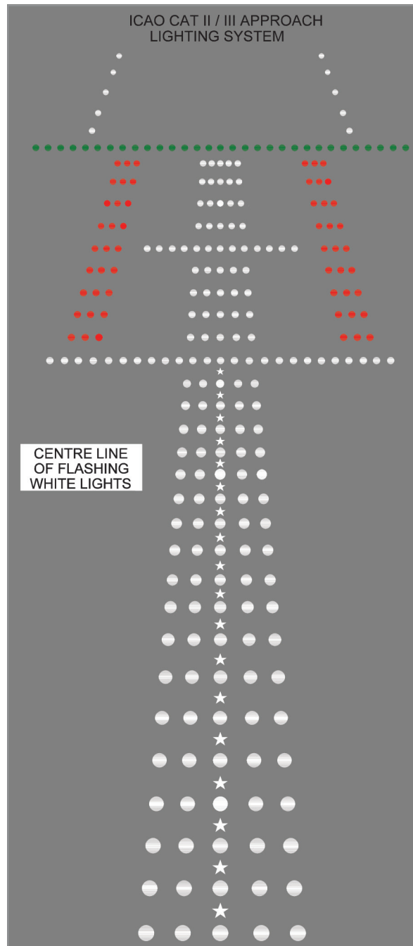
Figure 21.5 ICAO Cat II/III approach lighting system
