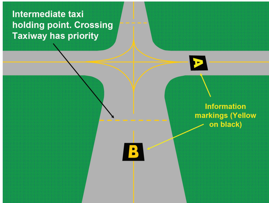
Figure 20.12 Intermediate holding position marking
