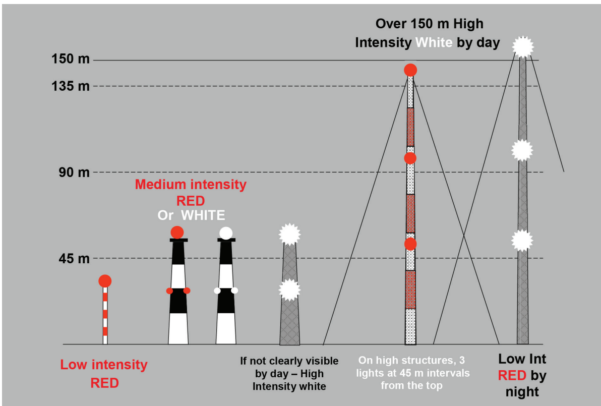
Figure 22.4 Methods of obstacle lighting
