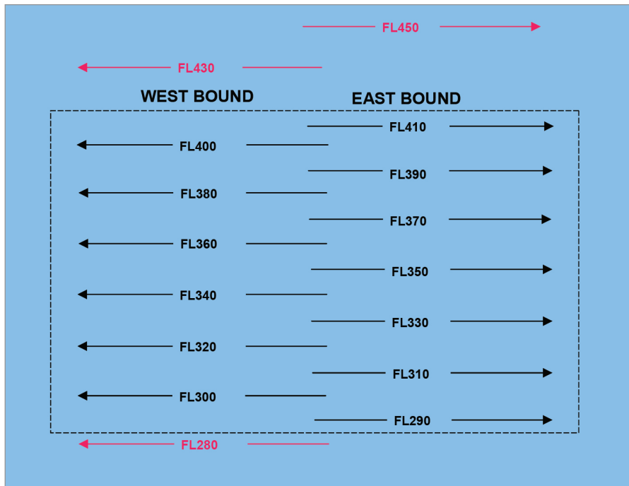
Figure 6.14 Reduced vertical separation minima
