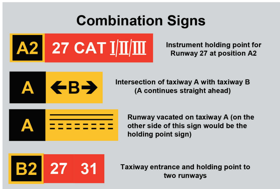
Figure 20.19 Combination signs
