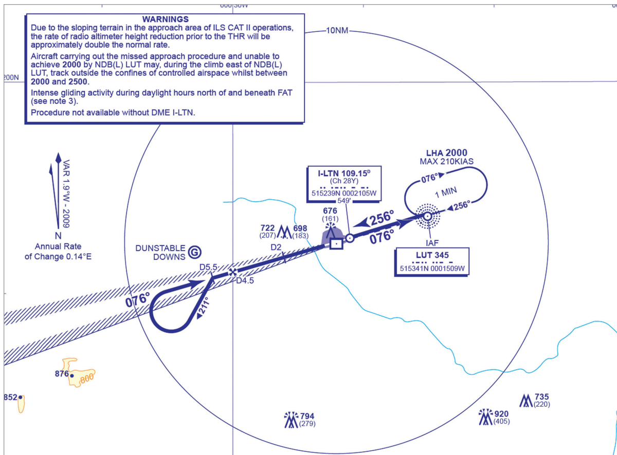
Figure 8.20 Procedure turn shown on an approach plate
