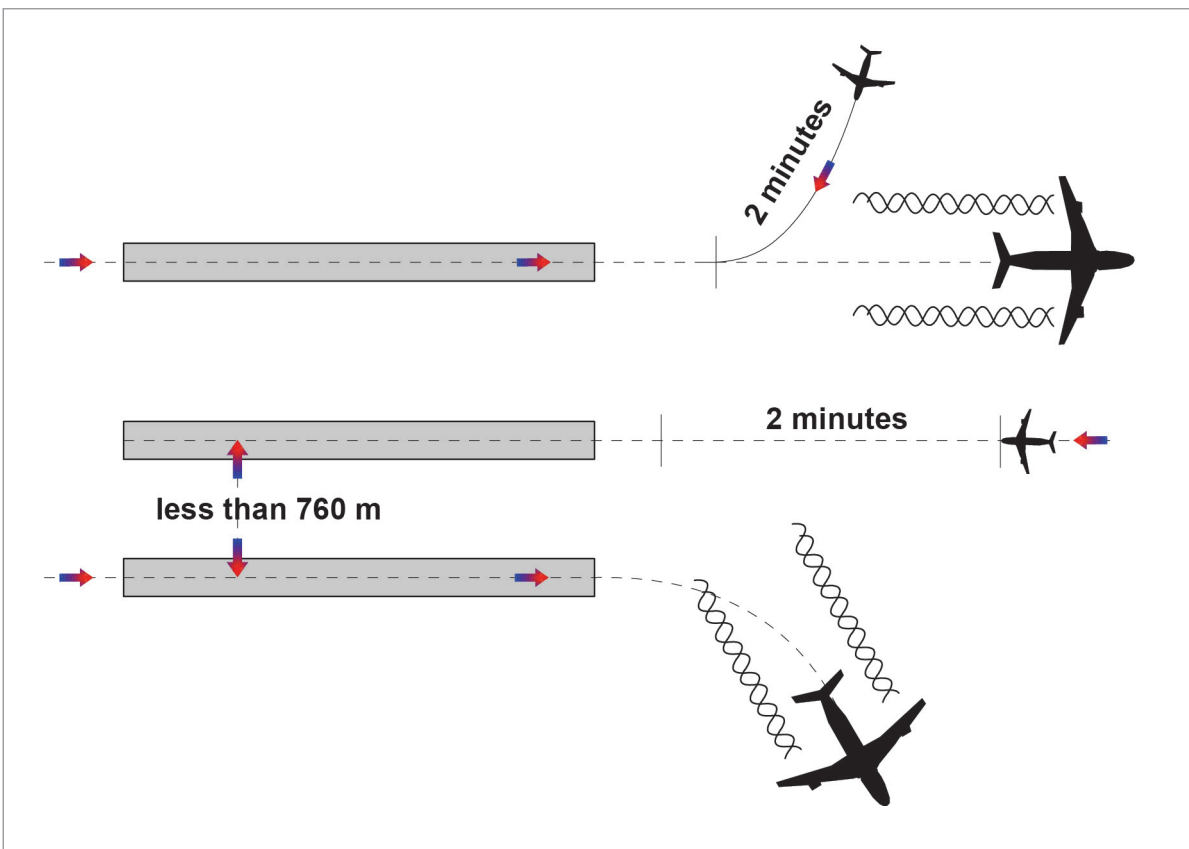
Figure 16.19 Opposite direction for landing
