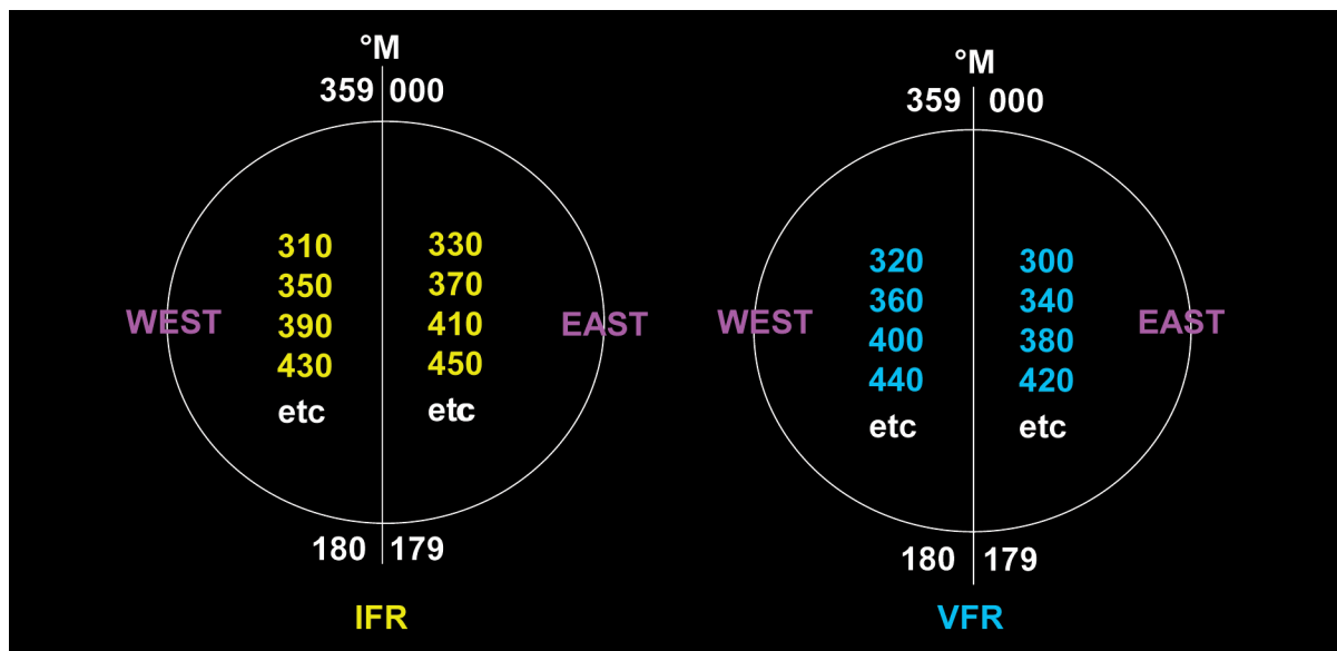
Figure 6.13 IFR and VFR flight levels above FL290
