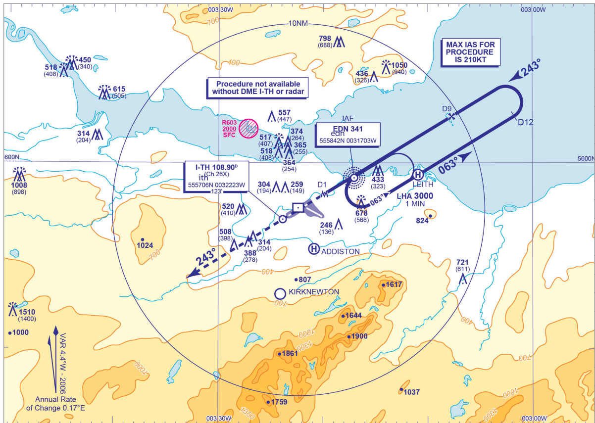
Figure 8.24 Racetrack shown on an approach plate
