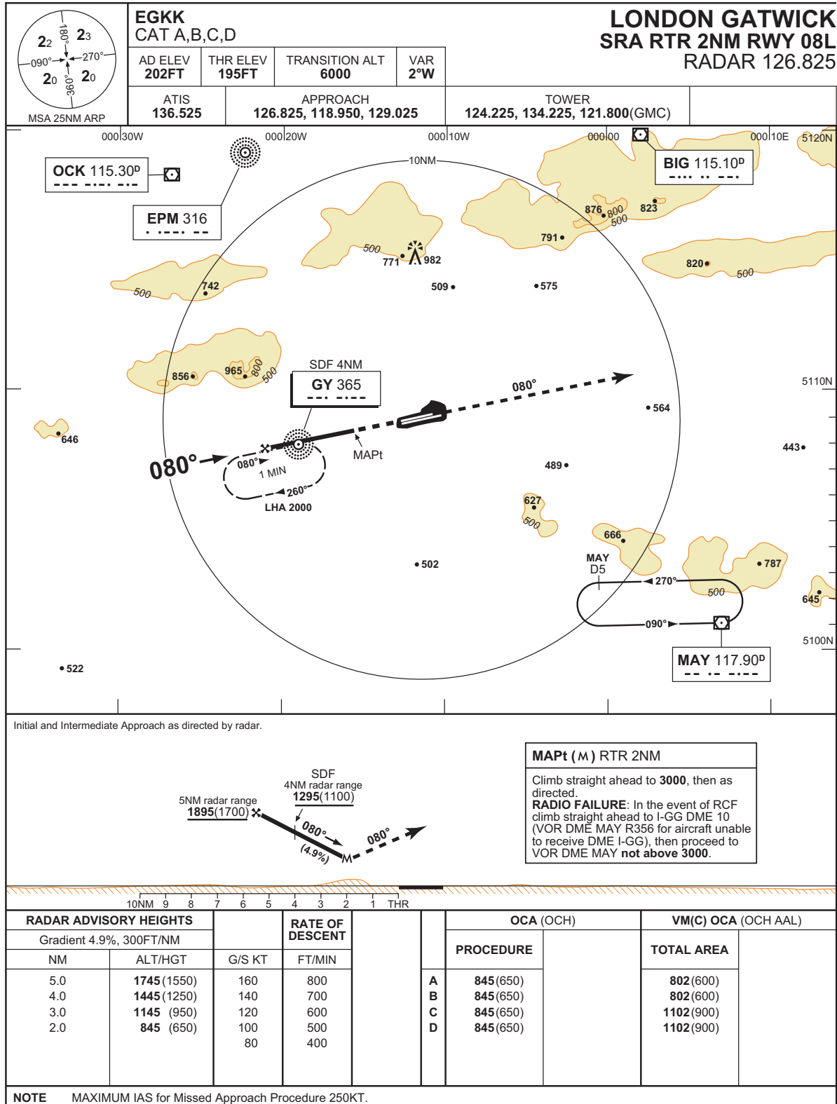
Figure 17.5 SRA approach
