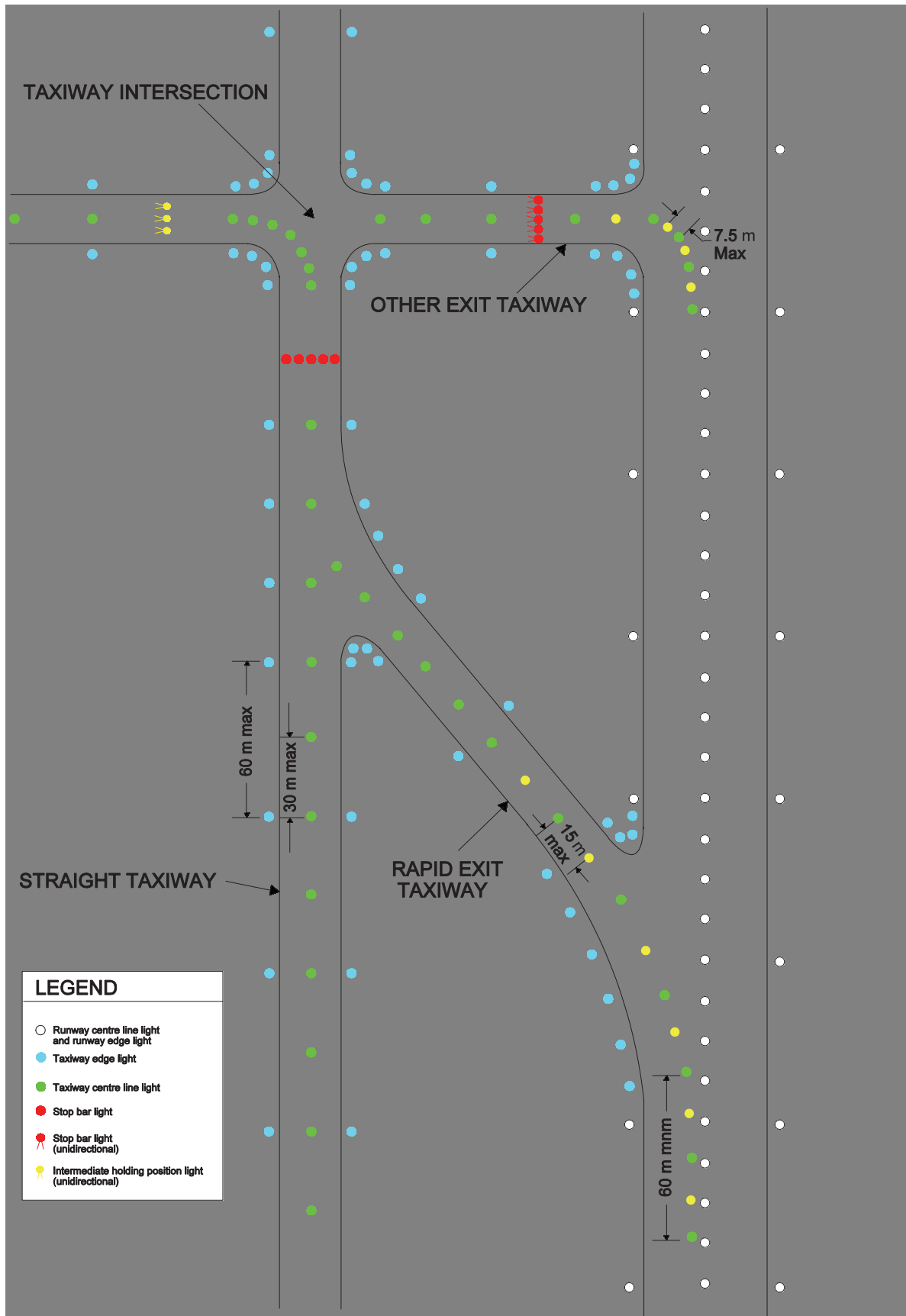
Figure 21.10 Arrangements of runway and taxiway lighting
