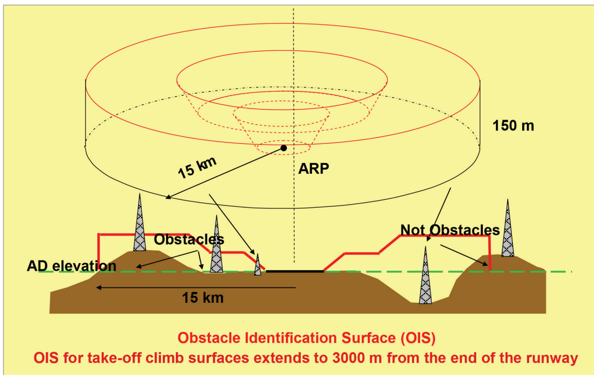
Figure 22.1 Obstacle identification surface (OIS)
