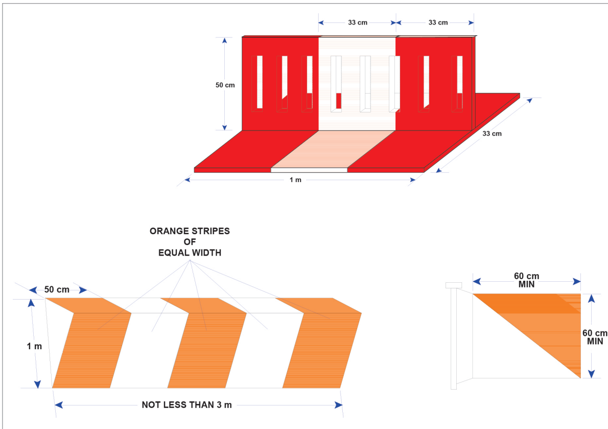
Figure 20.21 Boundary markers
