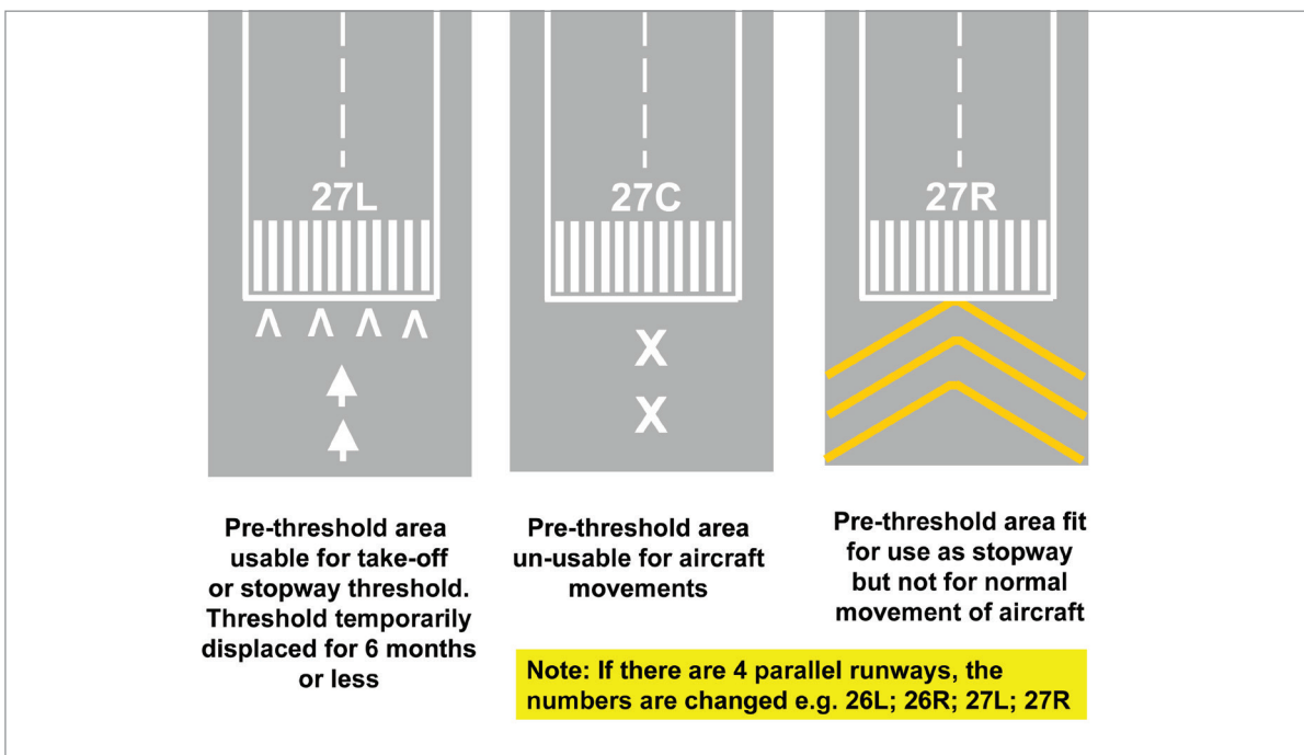
Figure 20.2 Runway designation markings
