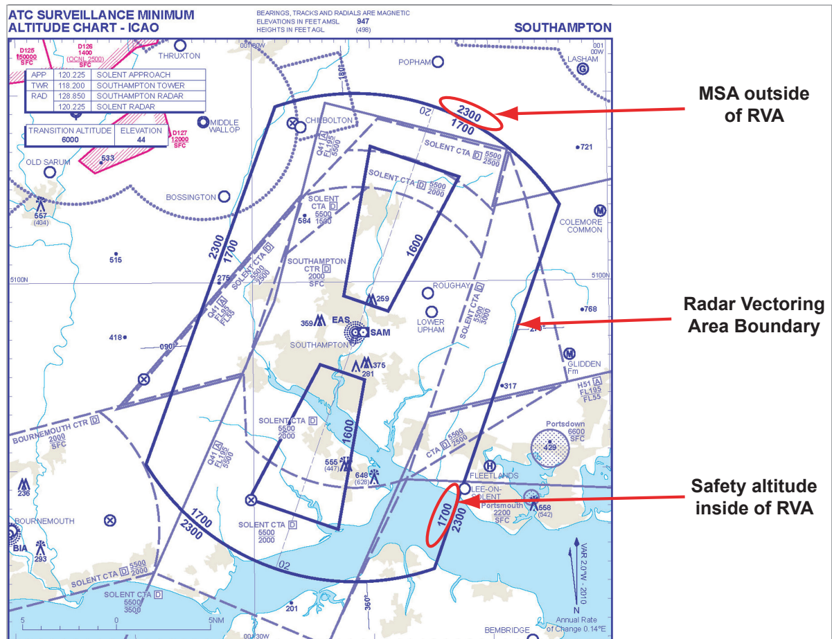
Figure 17.3 Radar vectoring area
