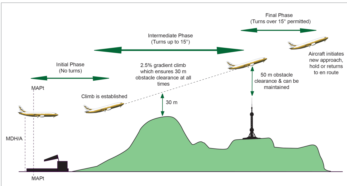
Figure 8.25 Three phases of the missed approach
