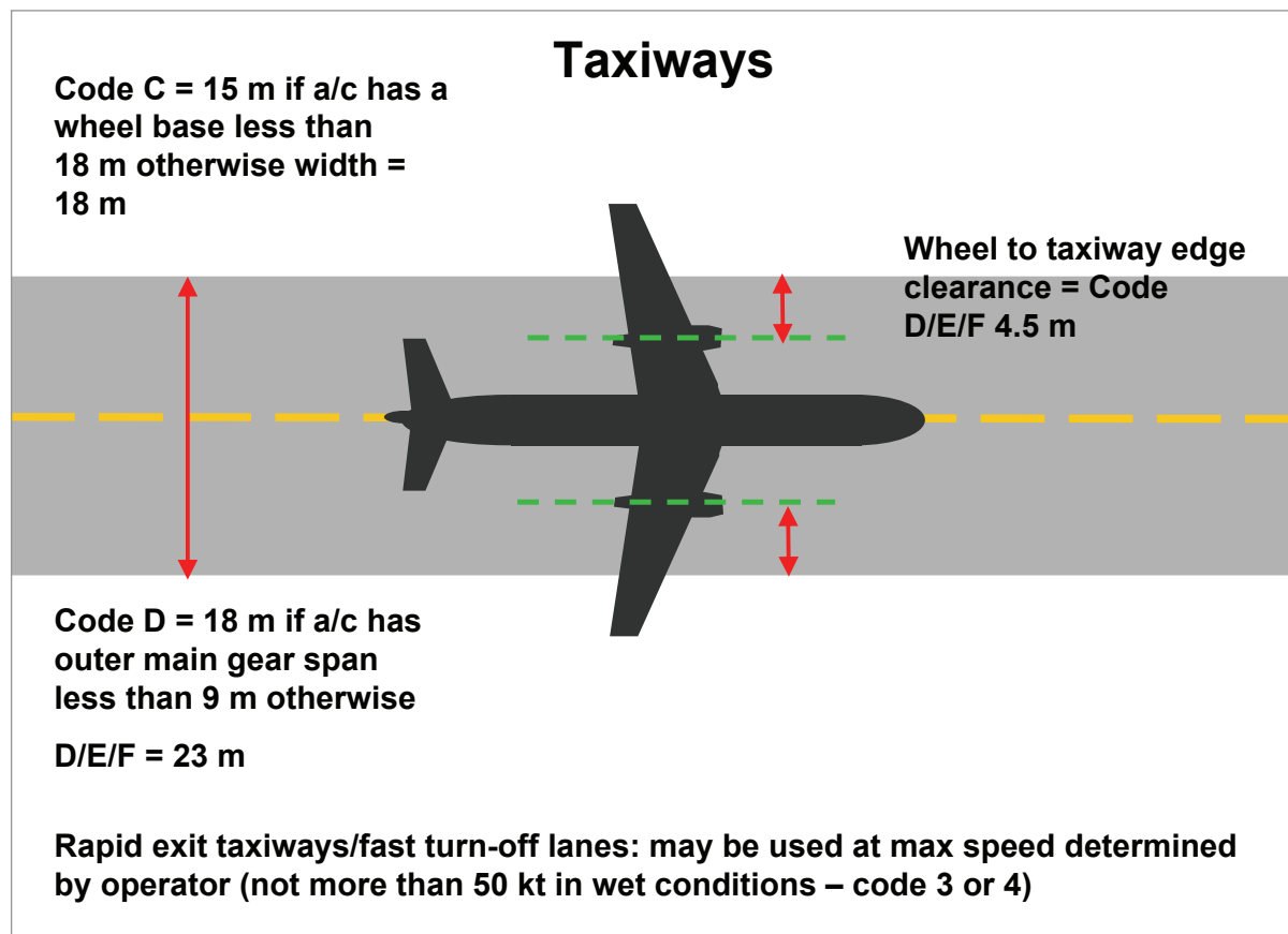
Figure 19.9: Taxiways
