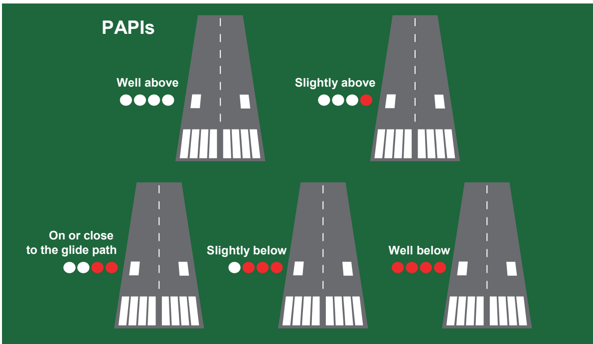
Figure 21.8 PAPI indications
