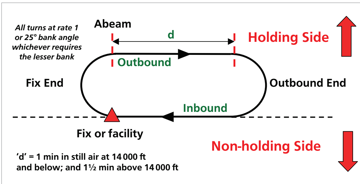
Figure 10.1 Holding pattern terminology
