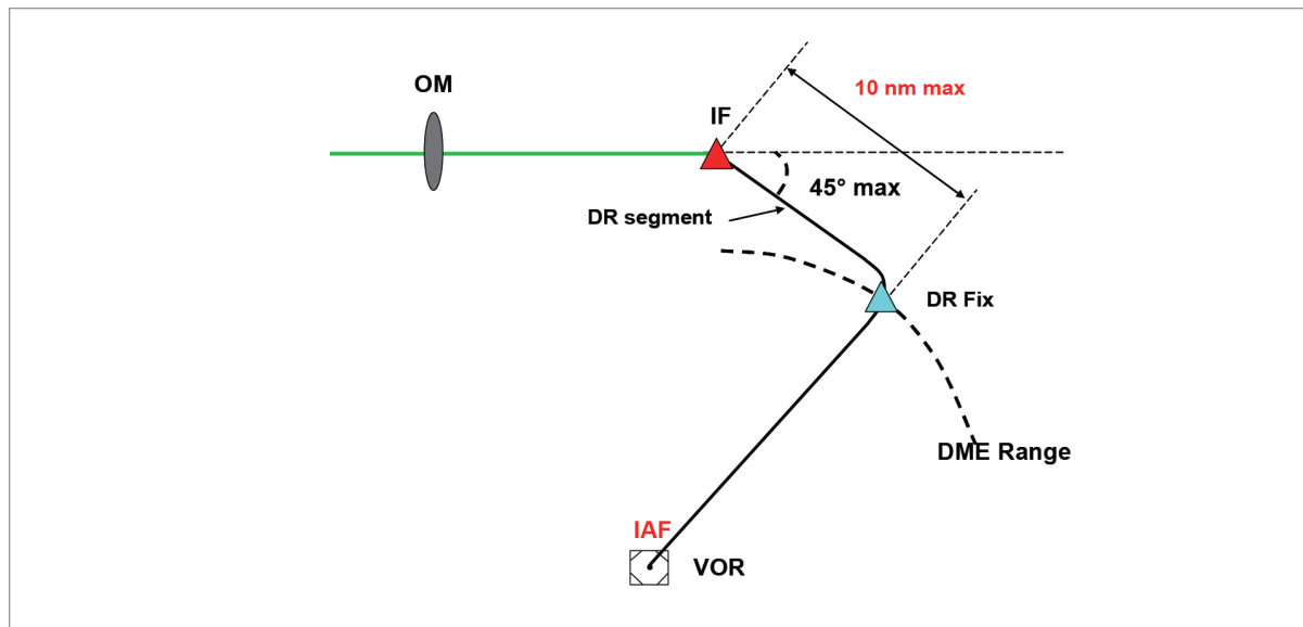
Figure 8.10 IAF to IF (DR segment)
