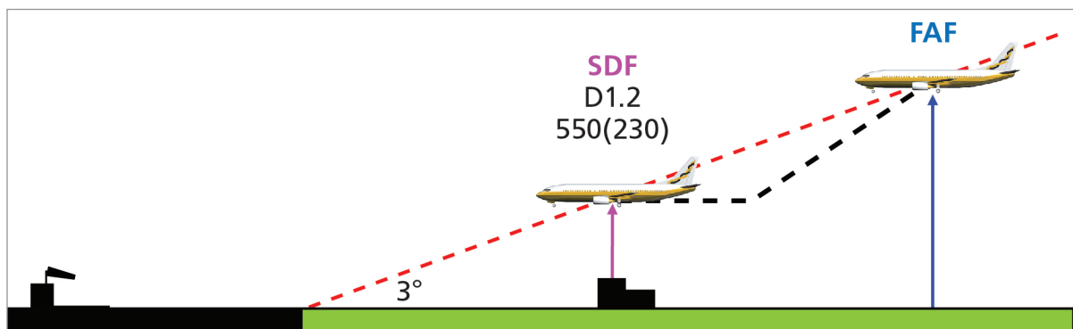
Figure 8.11 Step-down fix
