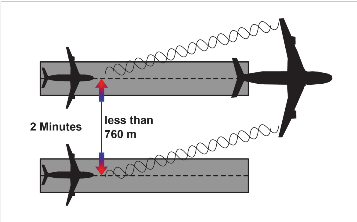
Figure 16.15 Parallel runways
