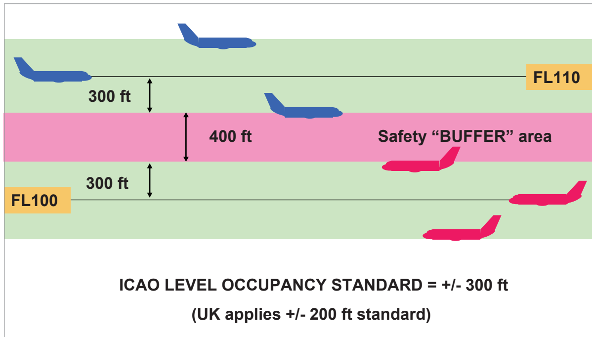
Figure 16.1 ICAO level occupancy standard
