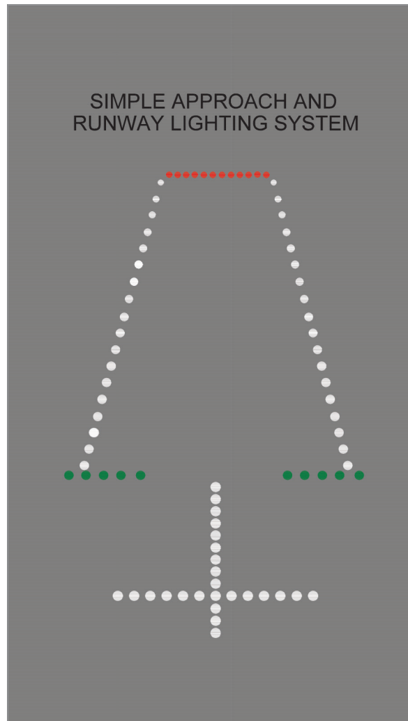
Figure 21.1 Simple approach lighting system
