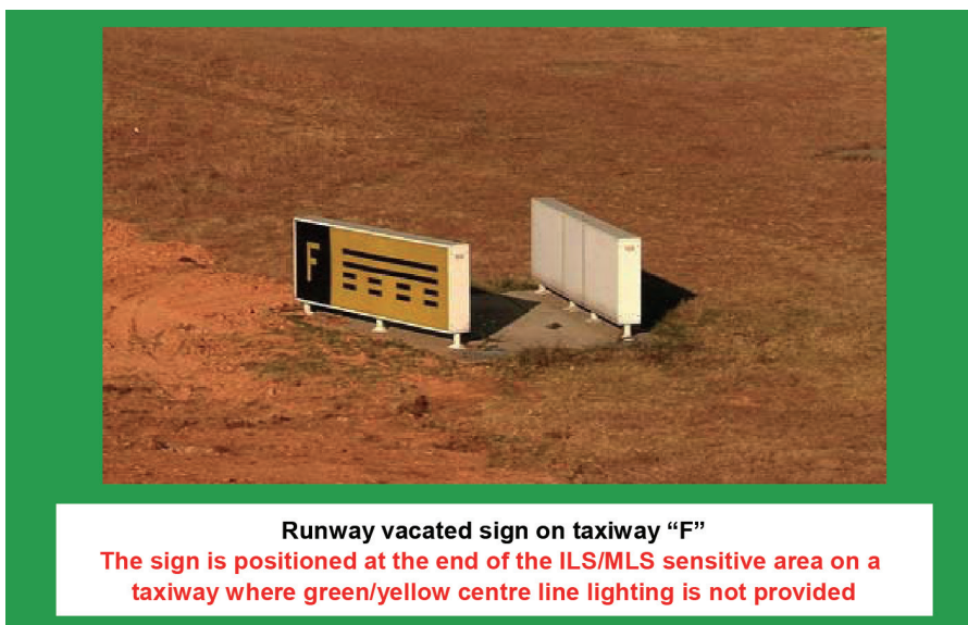
Figure 20.16 Runway vacated taxiway F
