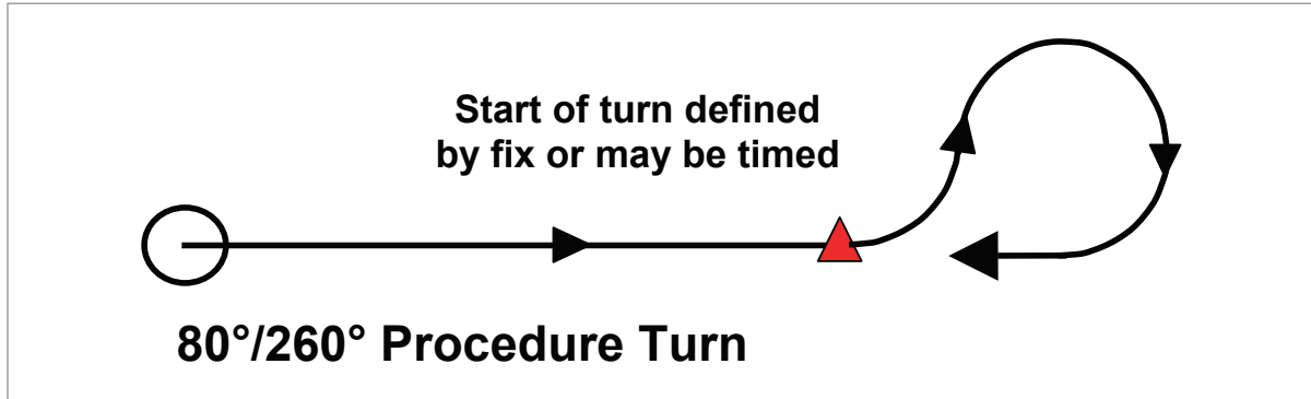
Figure 8.19 80°/260° - procedure turn
