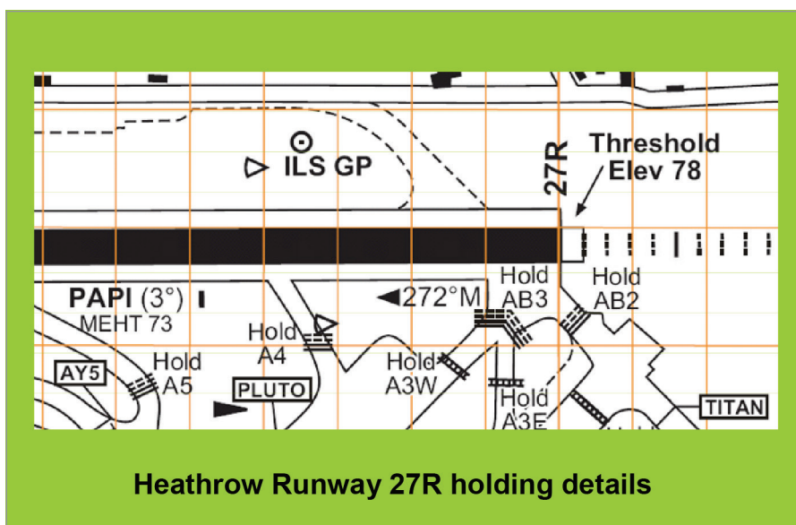
Figure 19.11 Holding points
