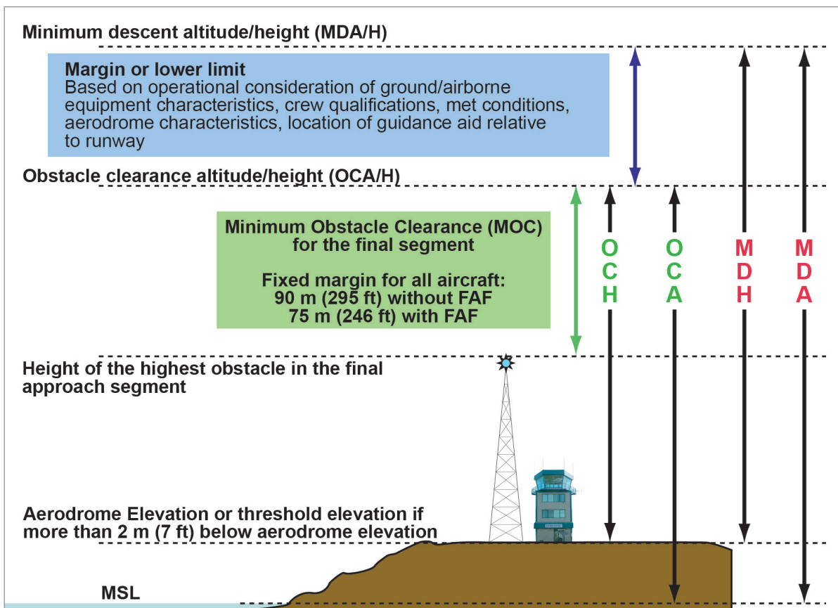
Figure 8.15 Method of determining MDA/MDH for non-precision approaches
