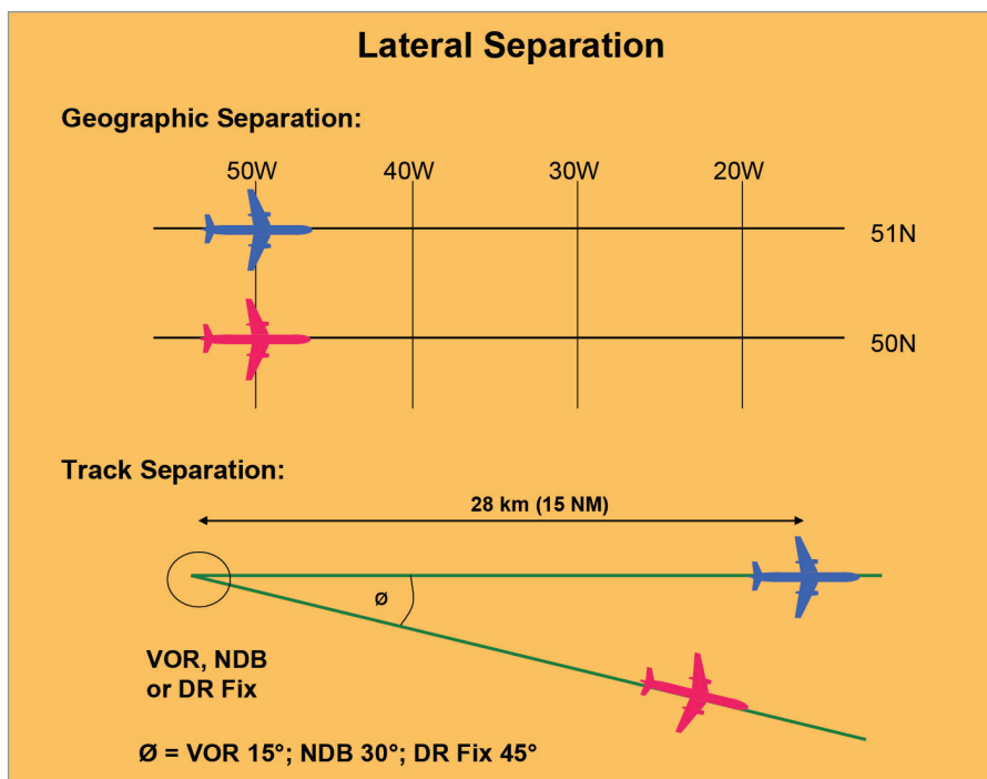
Figure 16.4 Lateral separation
