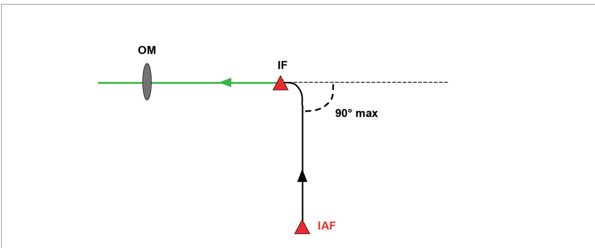
Figure 8.8 IAF to IF (precision approach)
