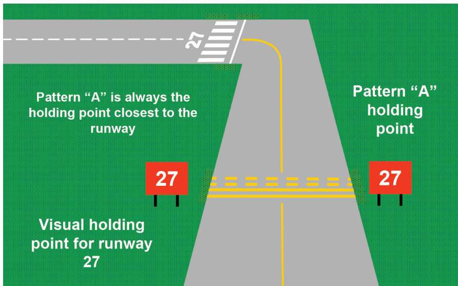
Figure 20.10 Runway holding markings, pattern A
