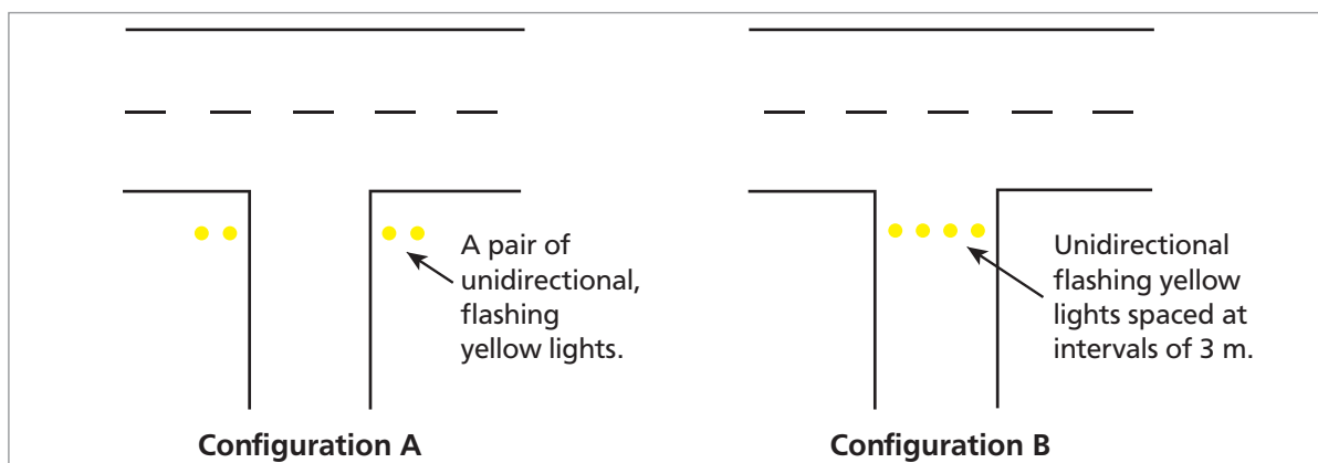
Figure 21.11 Runway and guard lights
