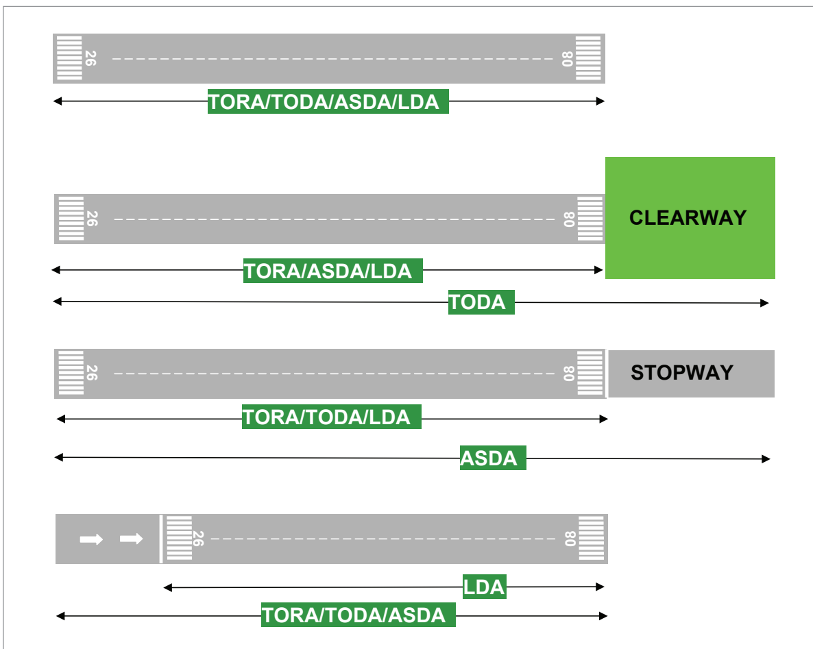
Figure 19.3 Declared distances
