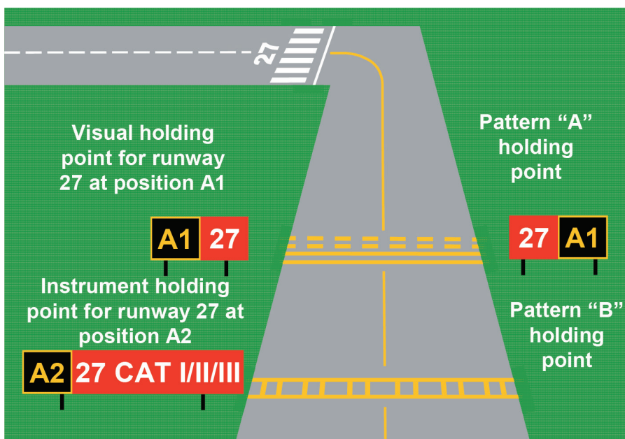
Figure 20.11 Runway holding markings, pattern B
