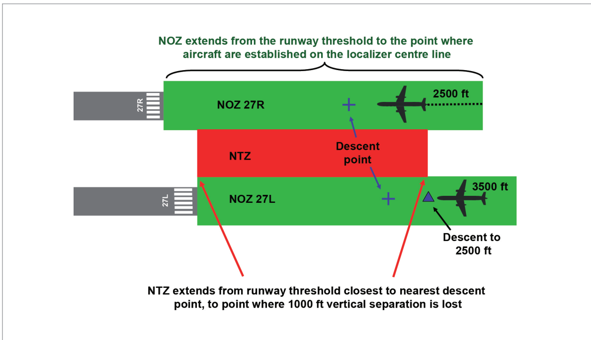
Figure 12.5 No transgression zone
