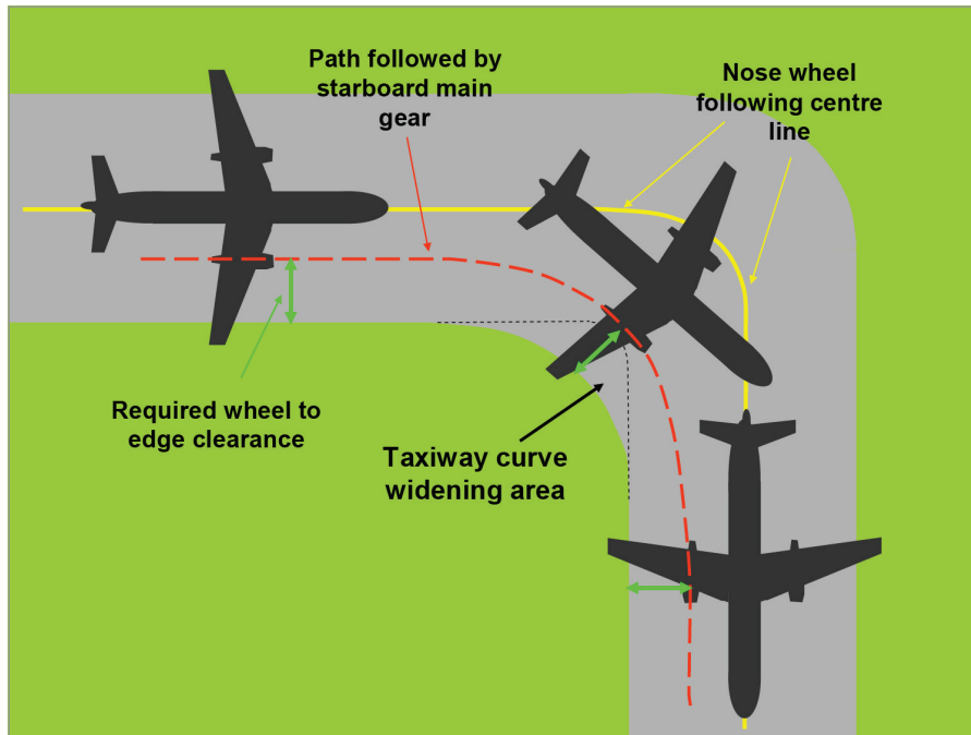
Figure 19.10: Taxiway curves
