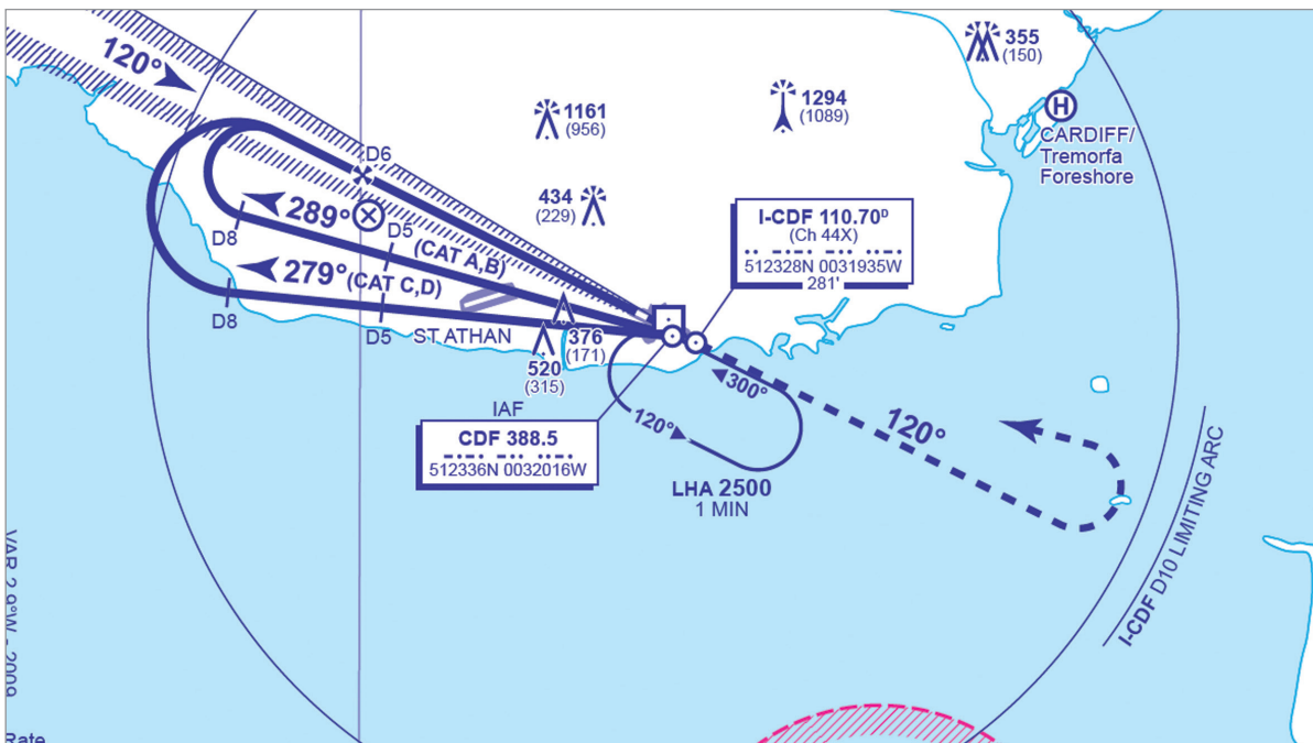
Figure 8.22 Base turn shown on an approach plate
