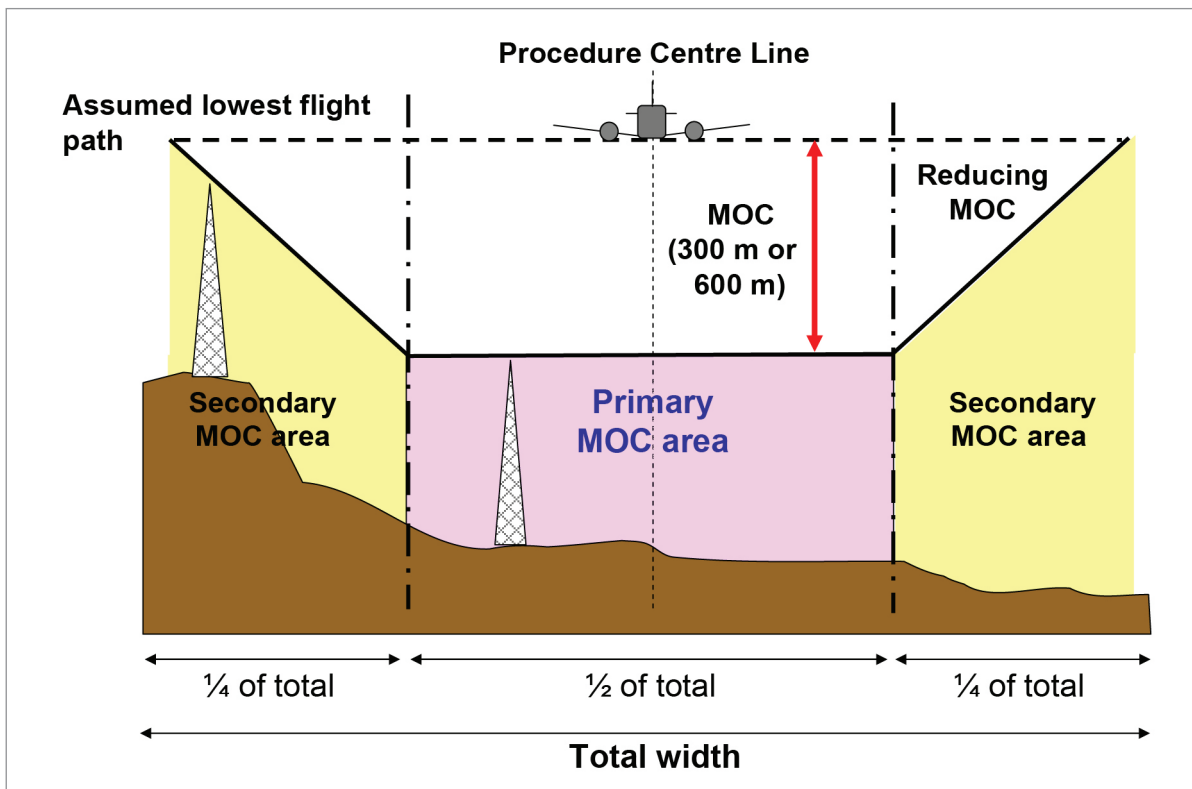
Figure 8.4 Characteristics of segments
