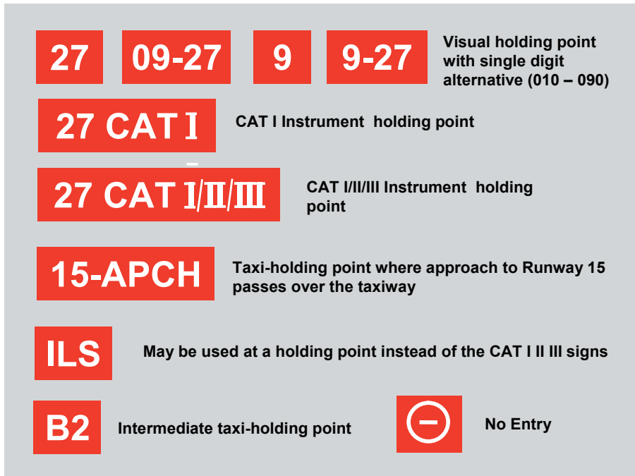
Figure 20.14 Sign characteristics
