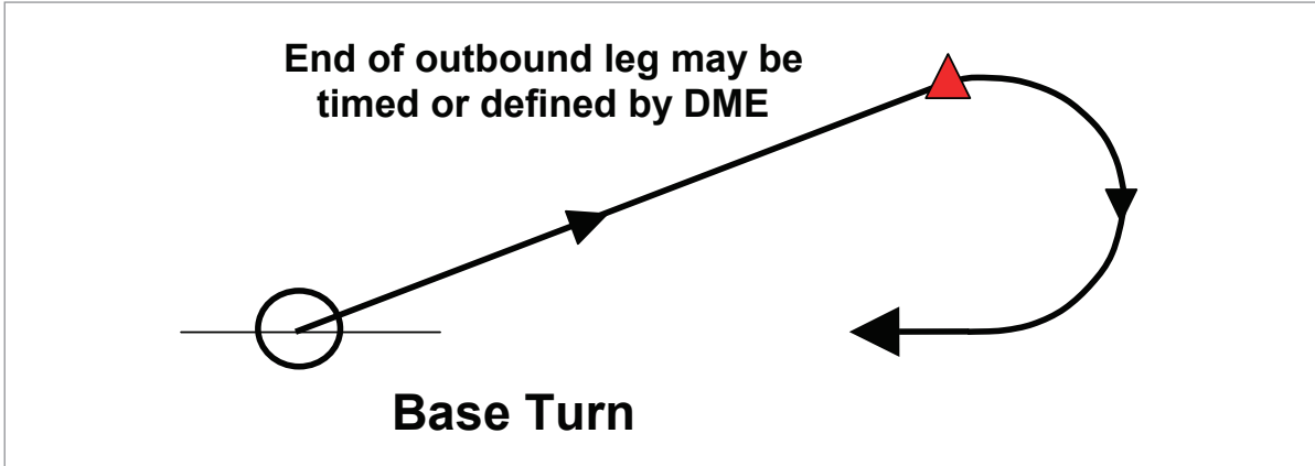
Figure 8.21 Base turn
