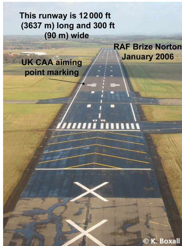
Figure 20.1 Runway markings at RAF Brize Norton
