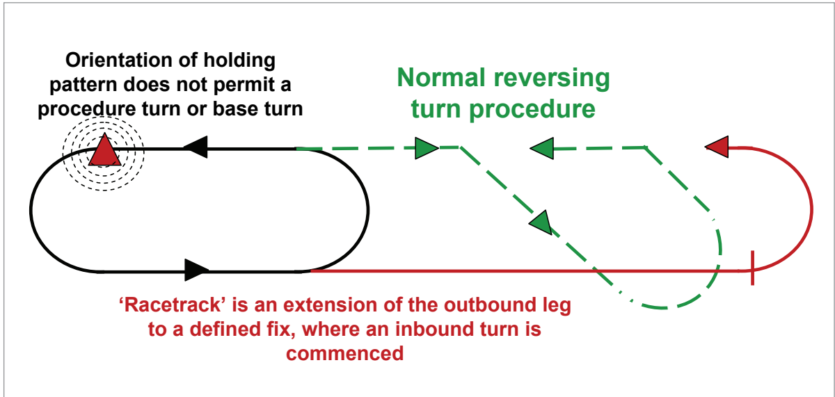
Figure 8.23 Racetrack procedure
