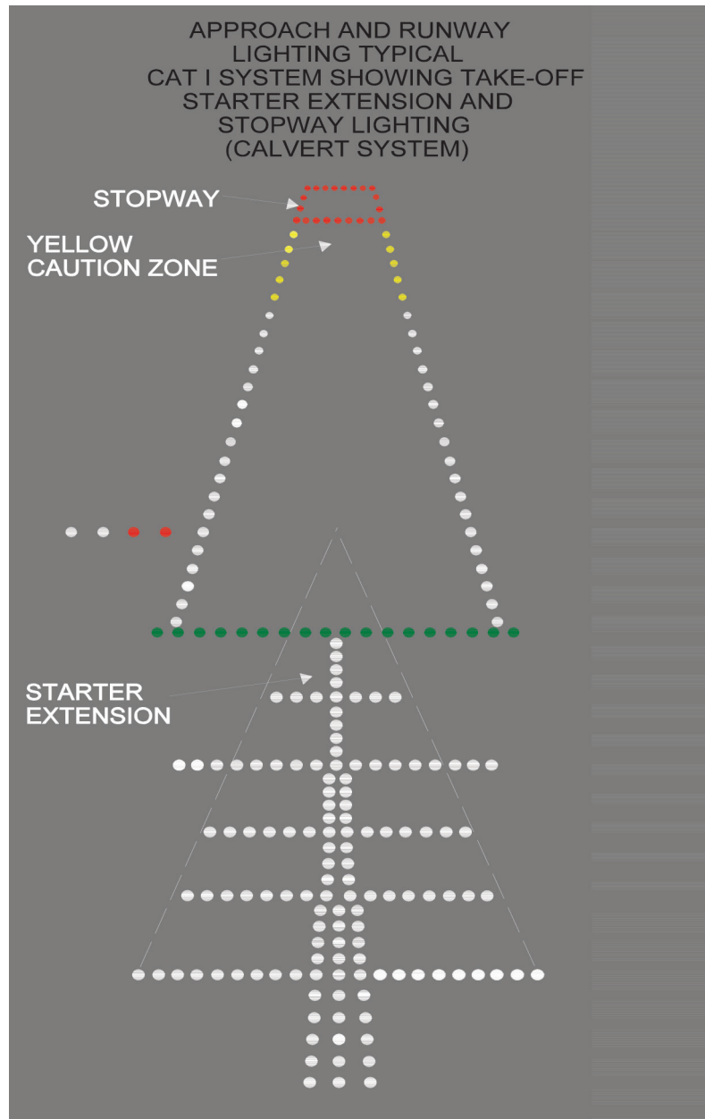
Figure 21.2 CAT I Calvert 5 bar and centre line system
