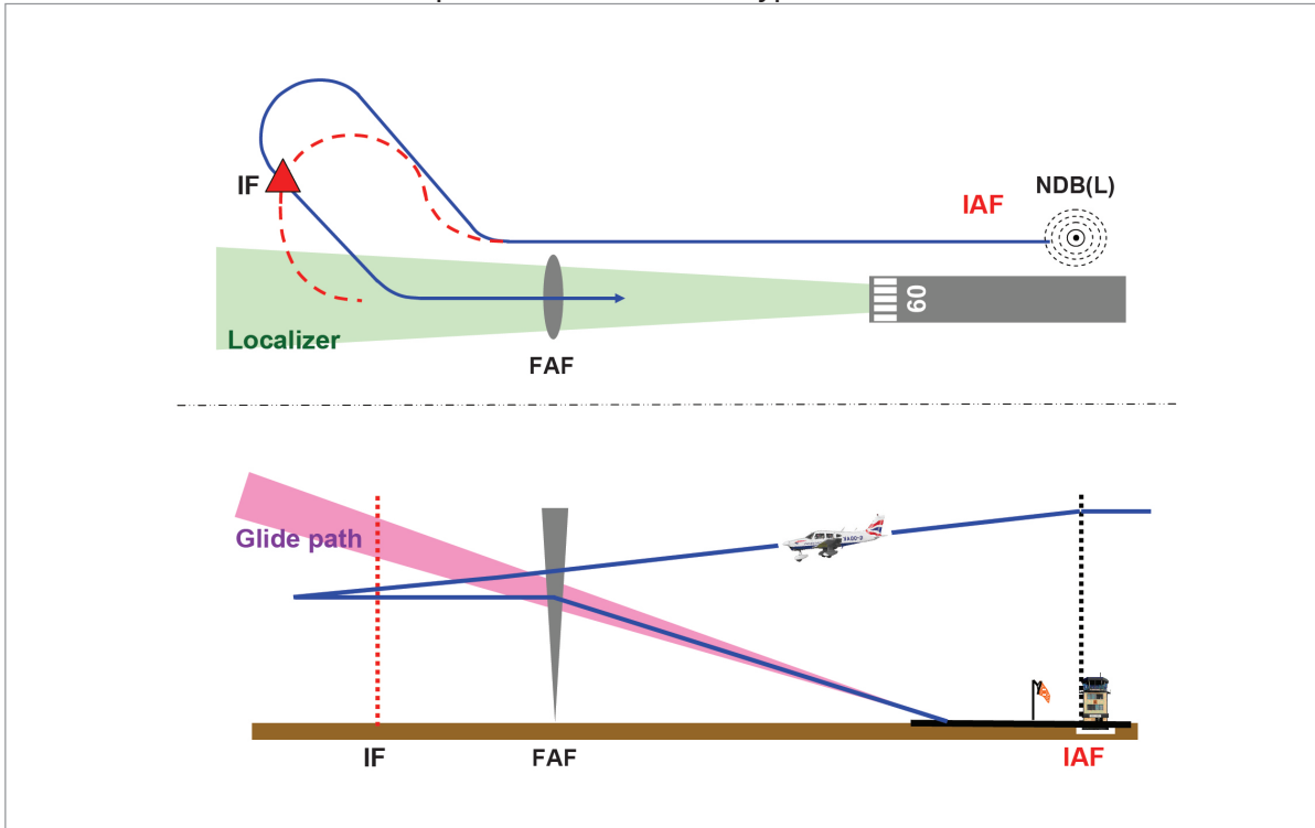
Figure 8.17 Track reversal - procedure turn
