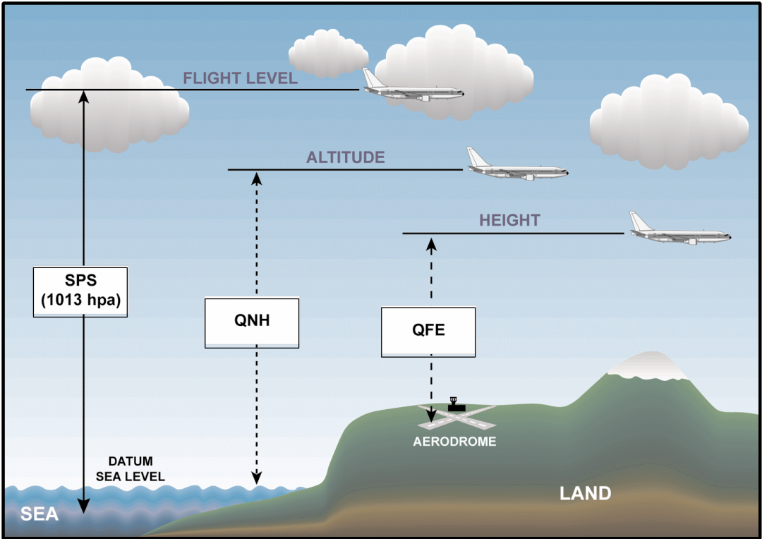
Pressure Settings
