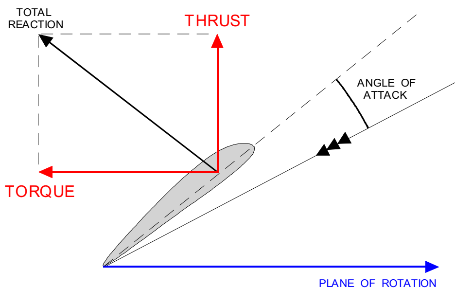
Figure 16.7 Thrust and Torque
