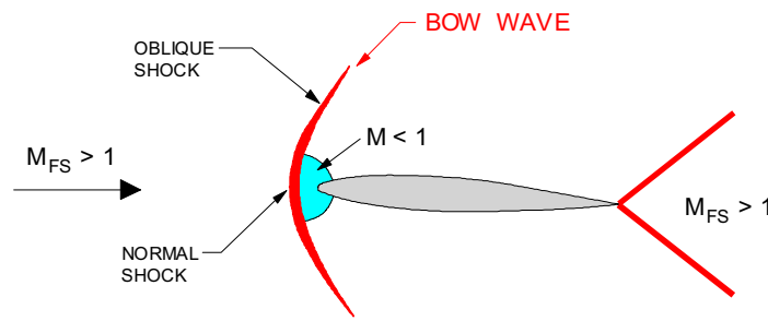
Figure 13.36 Bow Wave
