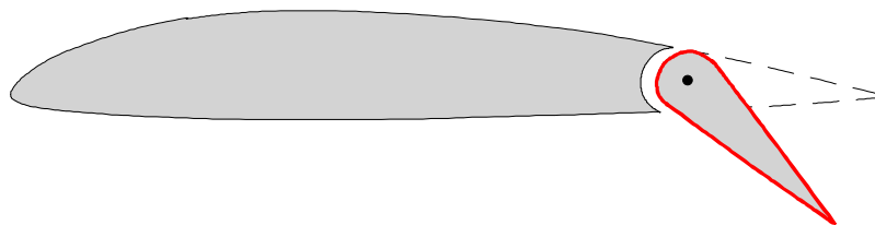
Figure 8.1 Plain Flap
