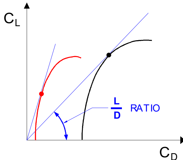
Figure 8.9 L/D Ratio
