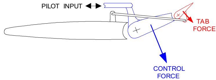
Figure 11.9 Anti-Balance Tab
