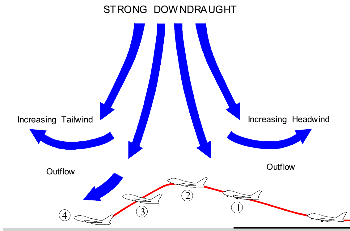
Figure 15.1 A Microburst Encounter During Take-Off
