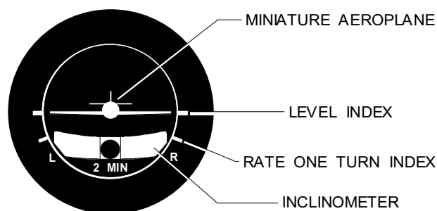
Figure 12.17 Turn Co-Ordinator
