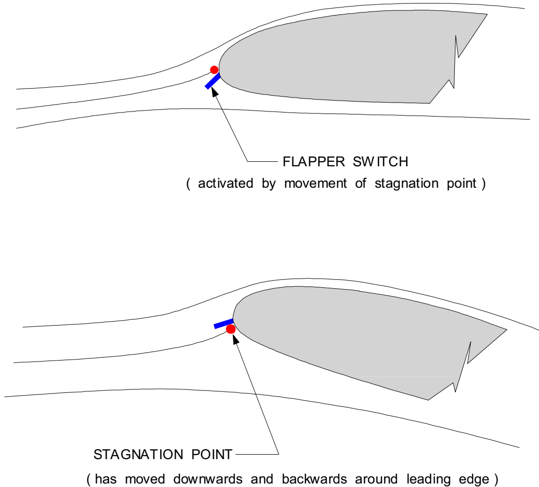
Figure 7.6. Flapper Switch
