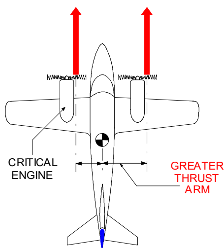
Figure 12.22 Critical Engine
