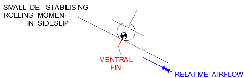
Figure 10.63a Ventral Fin Contribution
