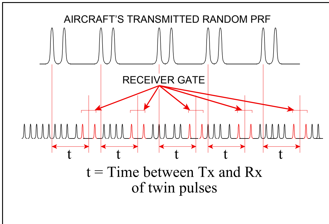
Figure 16.8 Acceptance of Own Pulses
