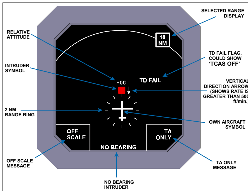
Figure 15.6 TCAS PPI
