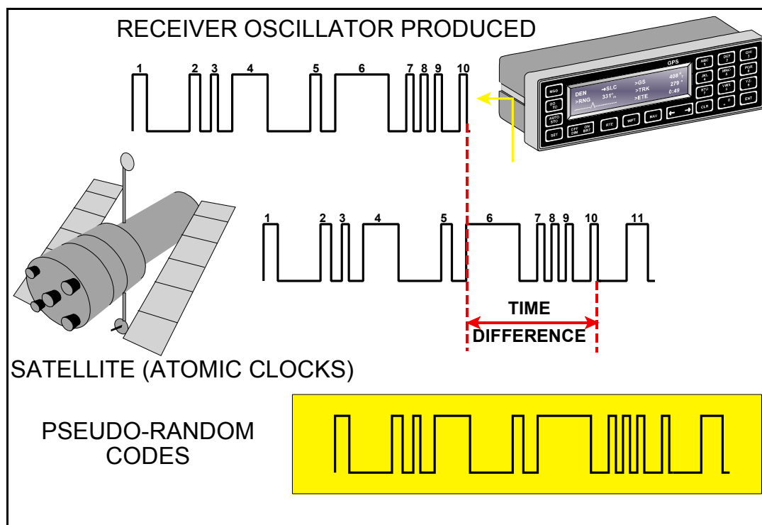
Figure 19.12 Pseudo-Random Code Time Measurement
