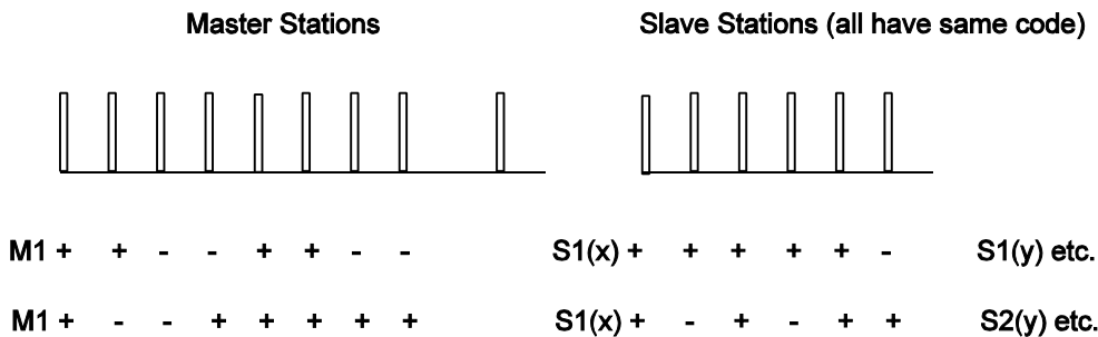
Figure 20.12b Phase Coding
