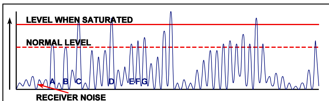
Figure 16.9 Beacon Saturation
