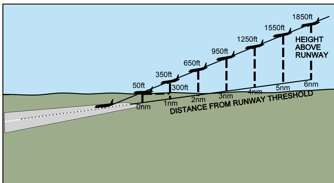
Figure 12.5 SRA Approach
