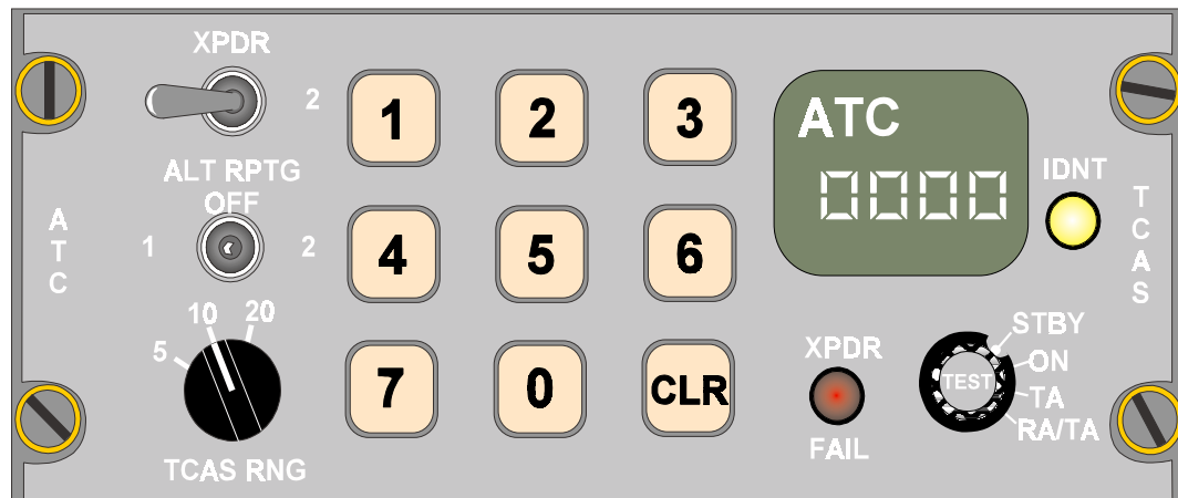
Figure 4.8 ATC Transponder/TCAS Control Panel
