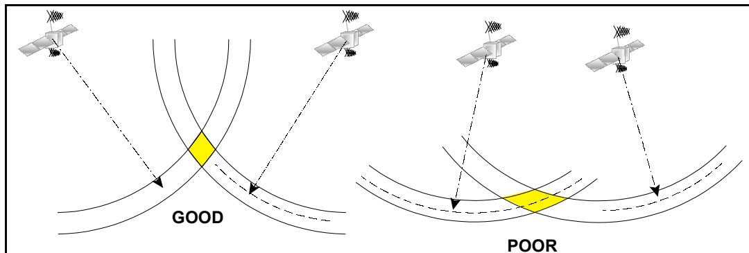
Figure 19.17 GDOP
