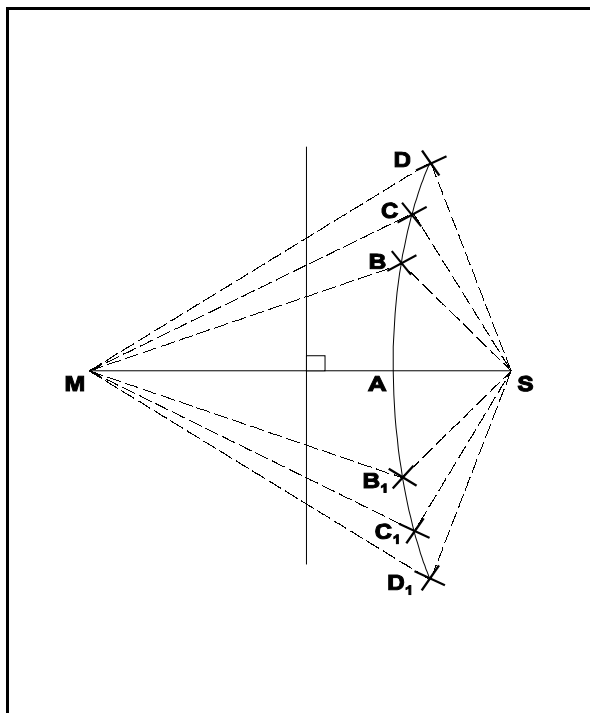
Figure 20.4 Curved Hyperbola
