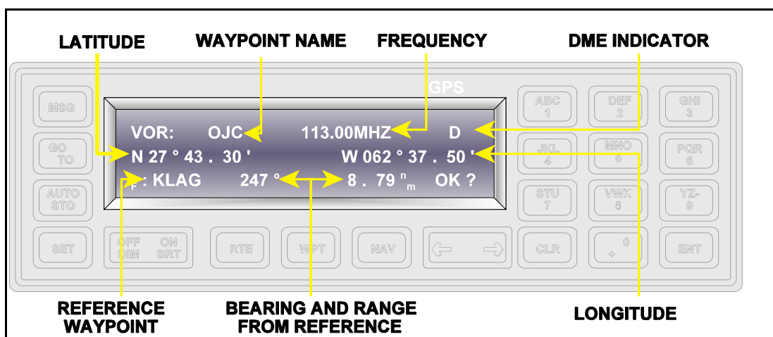
Figure 19.10d Waypoint Definitions Page
