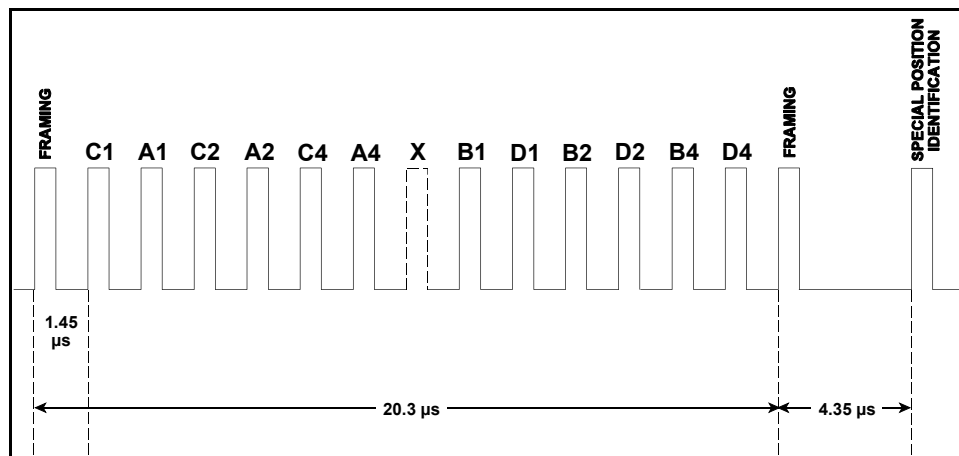
Figure 14.6 SSR Reply Pulse Patterns
