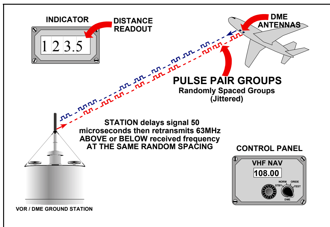
Figure 16.7 The Principle of Range Measurement
