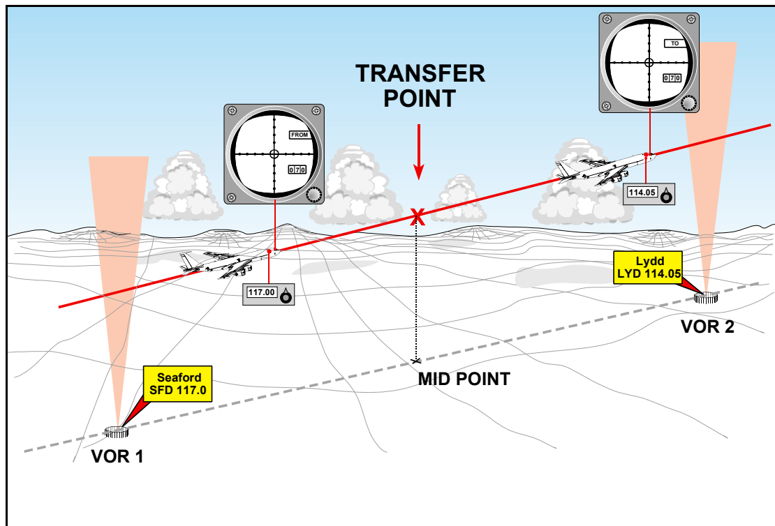
Figure 8.5 Tracking Between Two VORs
