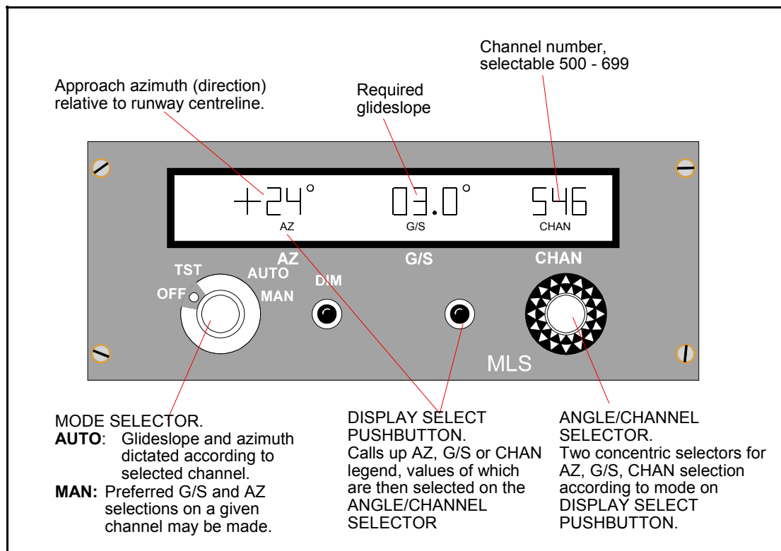
Figure 10.3 Typical MLS Flight Deck Control Panel
