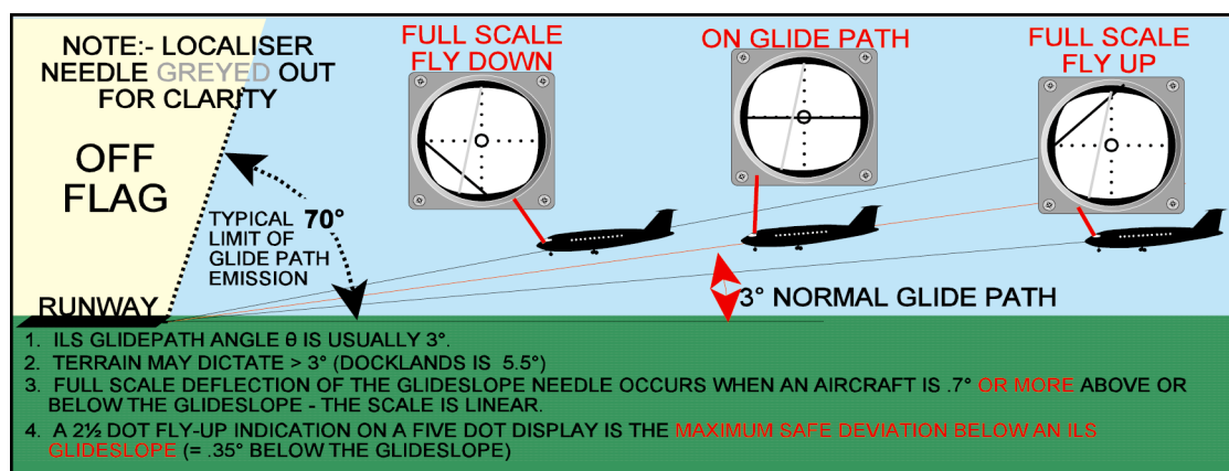
Figure 9.9 Glide Path
