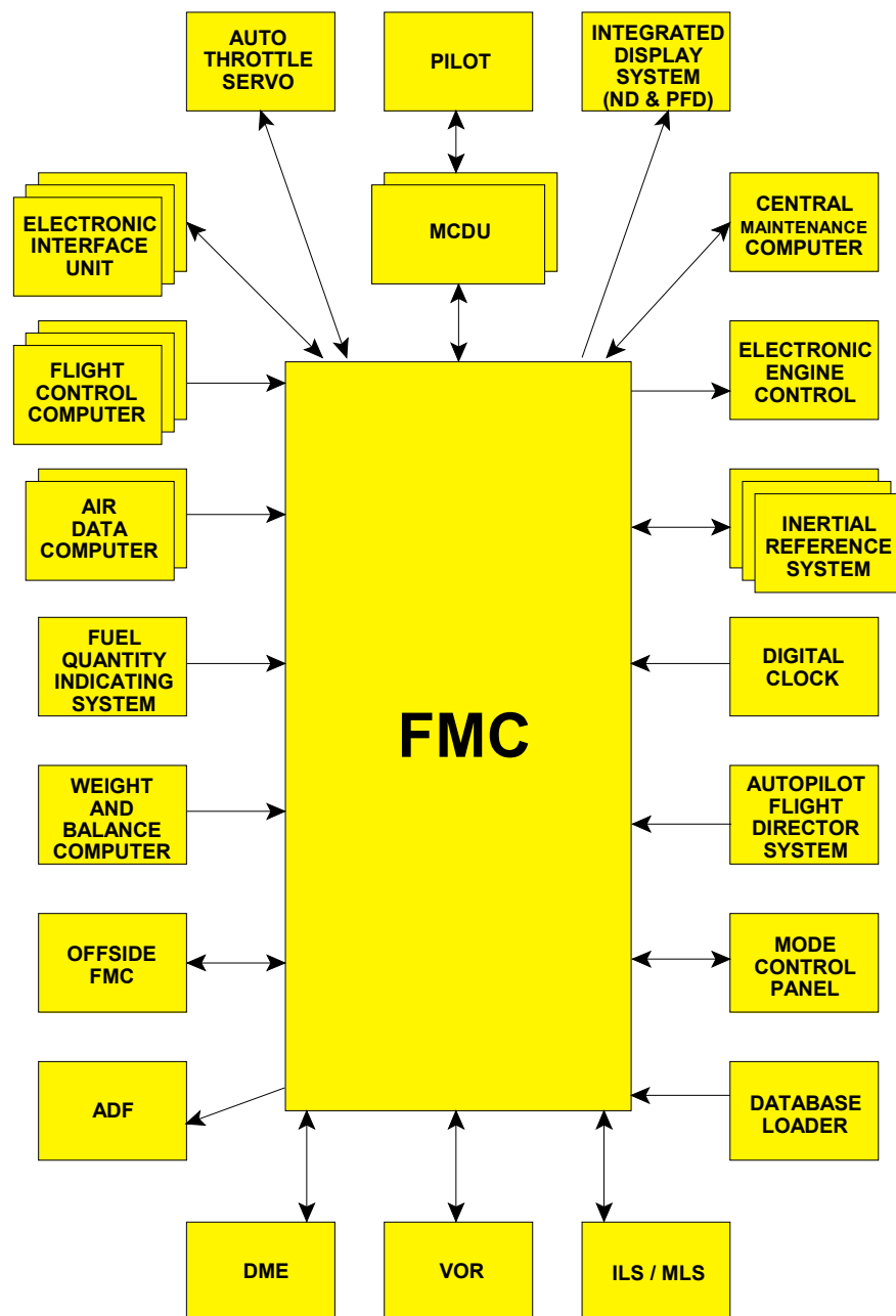
Figure 17.4 FMS Schematic
