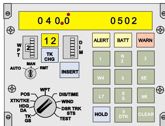
Figure 17.18 TK / GS (Track and Groundspeed)
