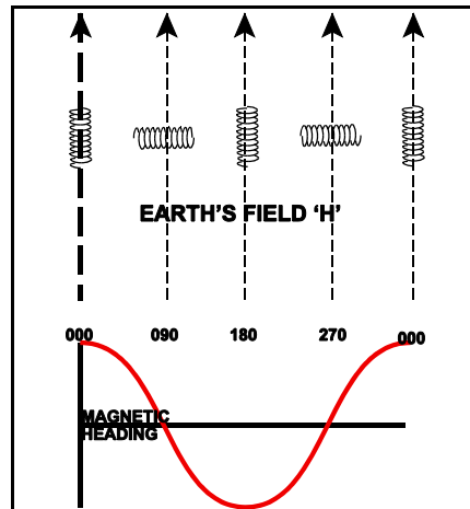
Figure 16.10 Effect of Earth's field on different directions of flux valve leg
