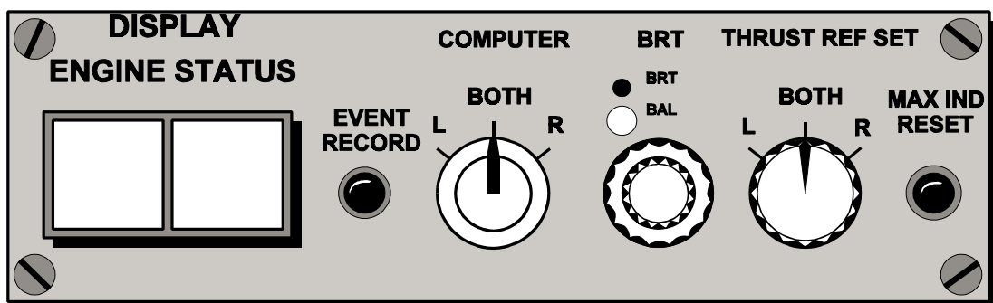
Figure 40.3 EICAS Display Select Panel
