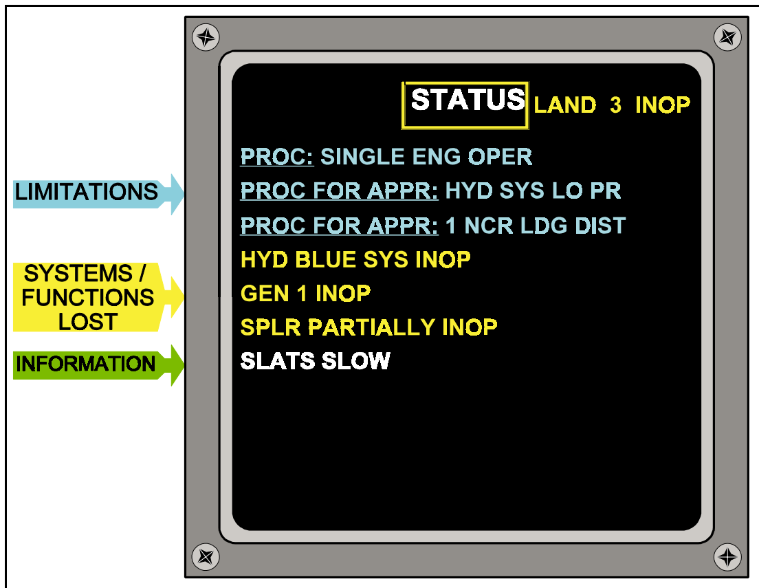
Figure 40.12 An Example of the Status Display
