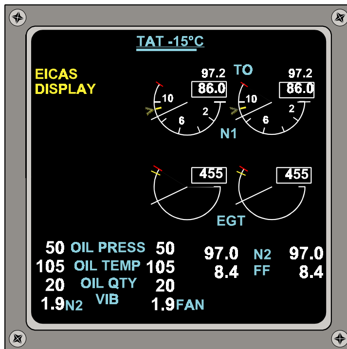
Figure 40.6 The 'Compact Format' Display
