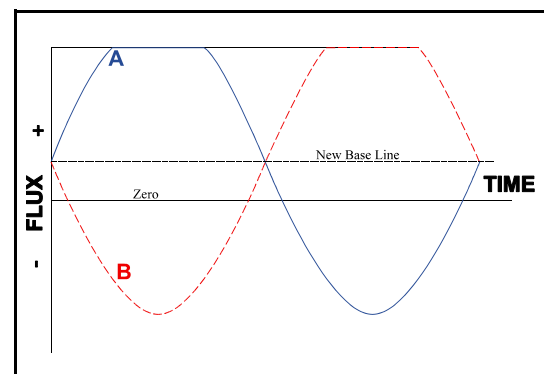
Figure 16.8 Effect of Earth's background magnetism
