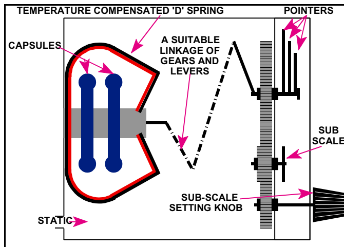
Figure 5.2 Sensitive Altimeter
