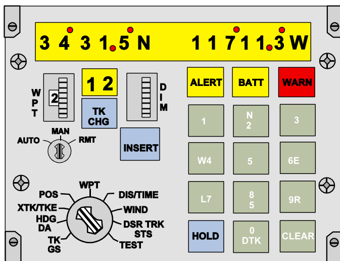
Figure 17.8 POS (Present Position)
