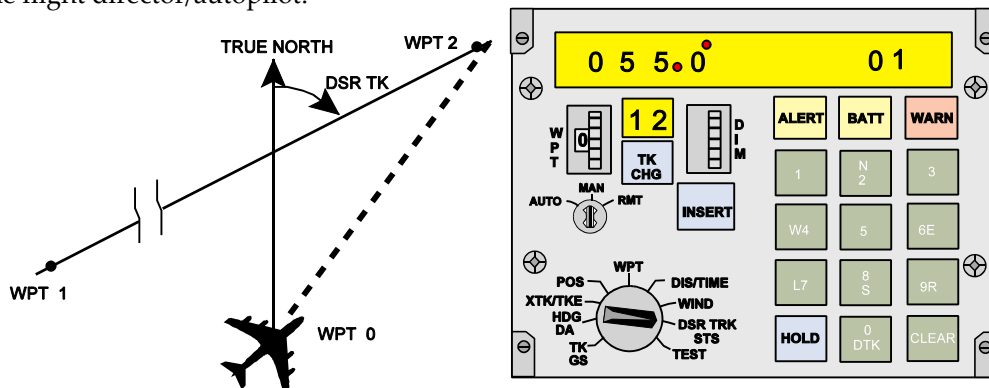
Figure 17.23 Waypoint Zero
