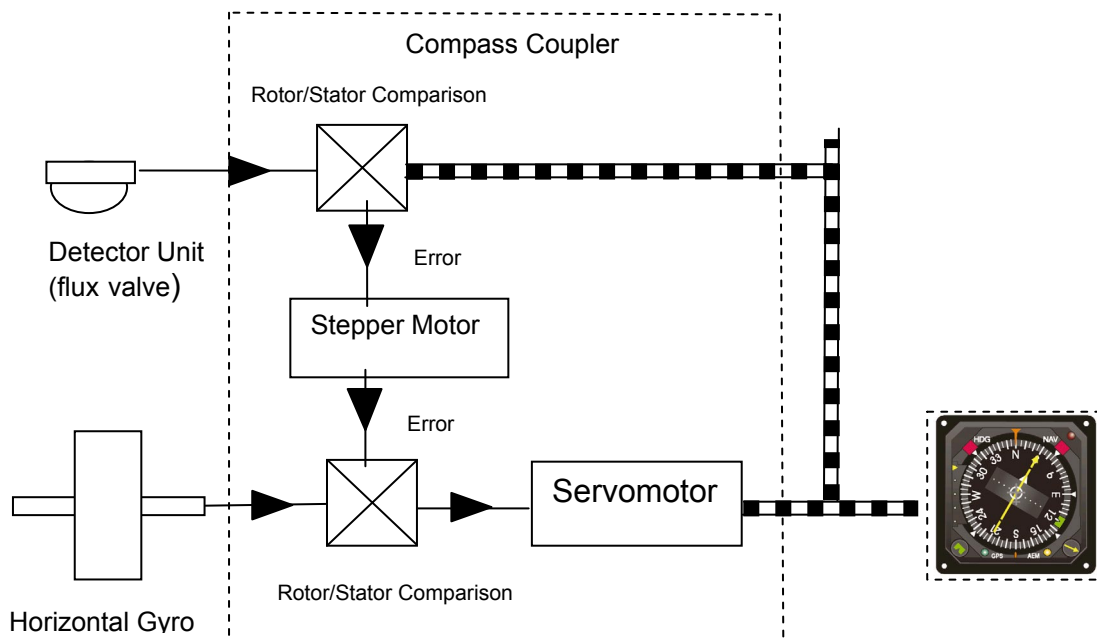
Figure 16.17 Remote System with Compass Coupler
