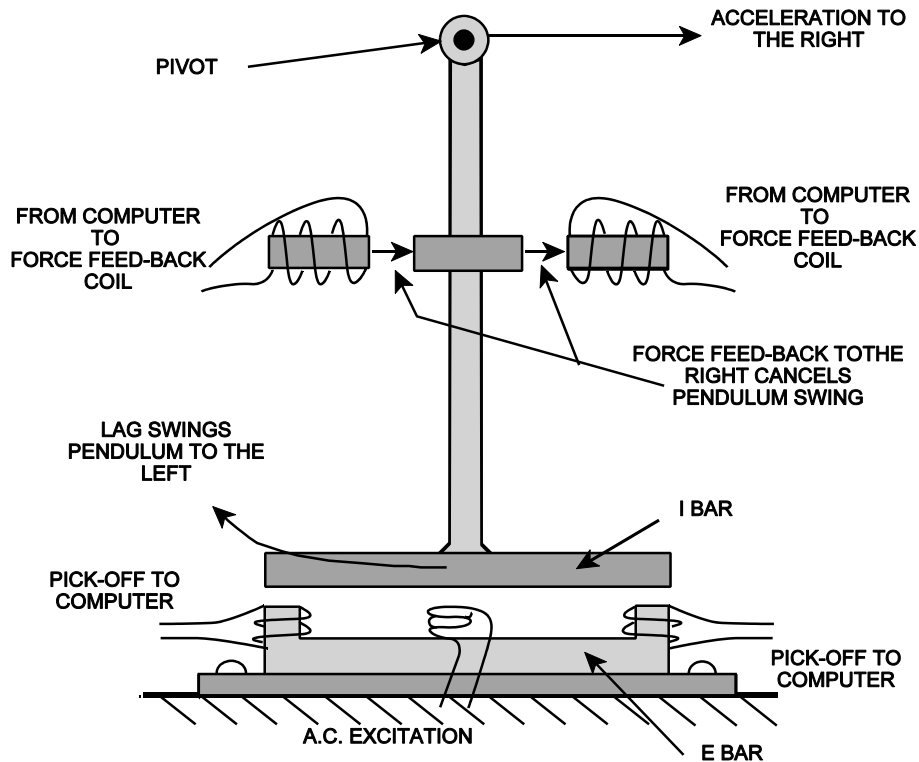
Figure 17.3 Accelerometer
