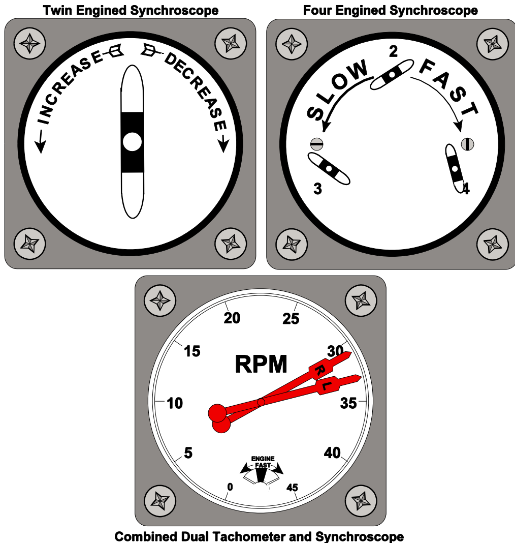
Figure 39.10 Synchrosopes
