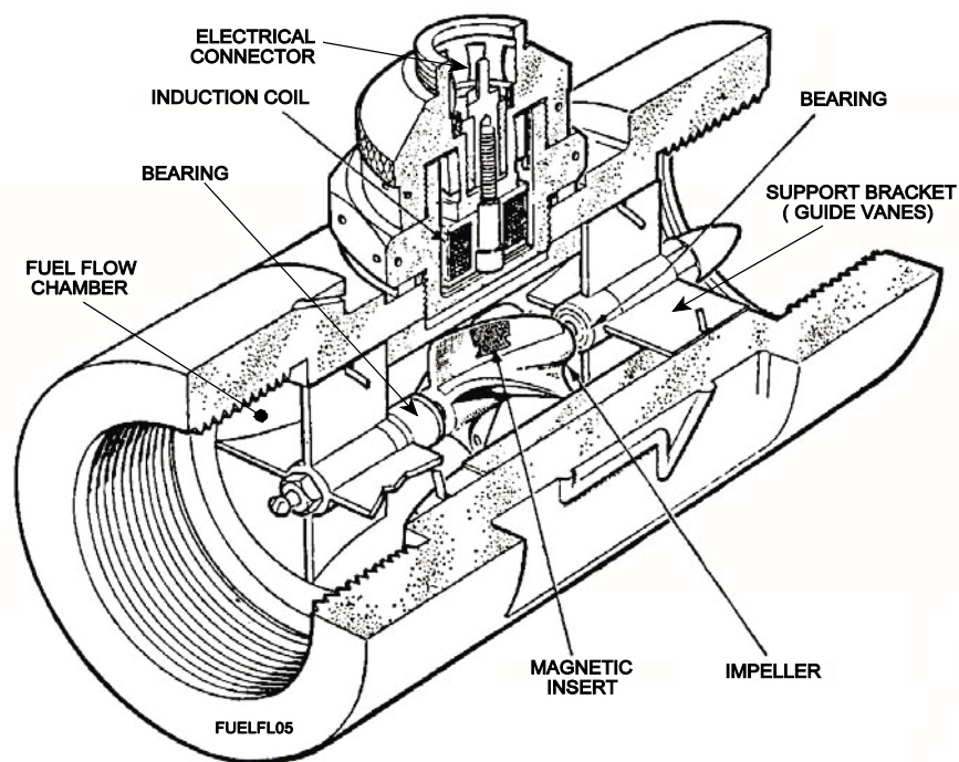
Figure 39.24 A typical Fuel Flowmeter
