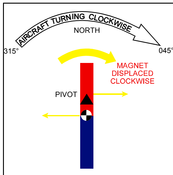
Figure 9.11 Turning from 315° to 045° (Northern Hemisphere)
