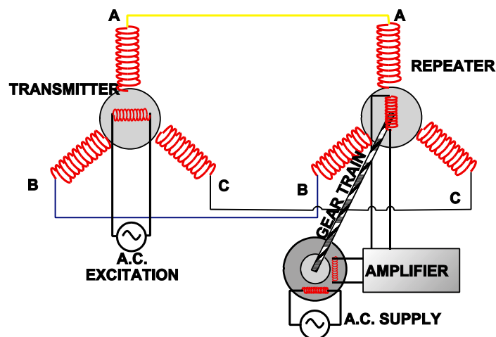
Figure 1.21 Synchro-Servo System
