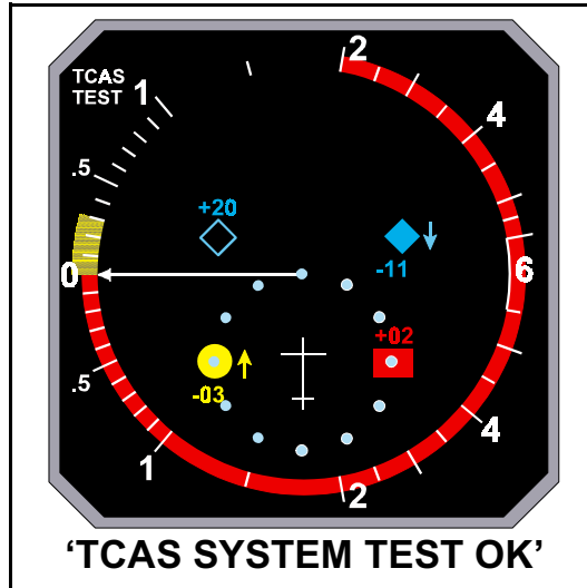
Figure 36.13 Test Display
