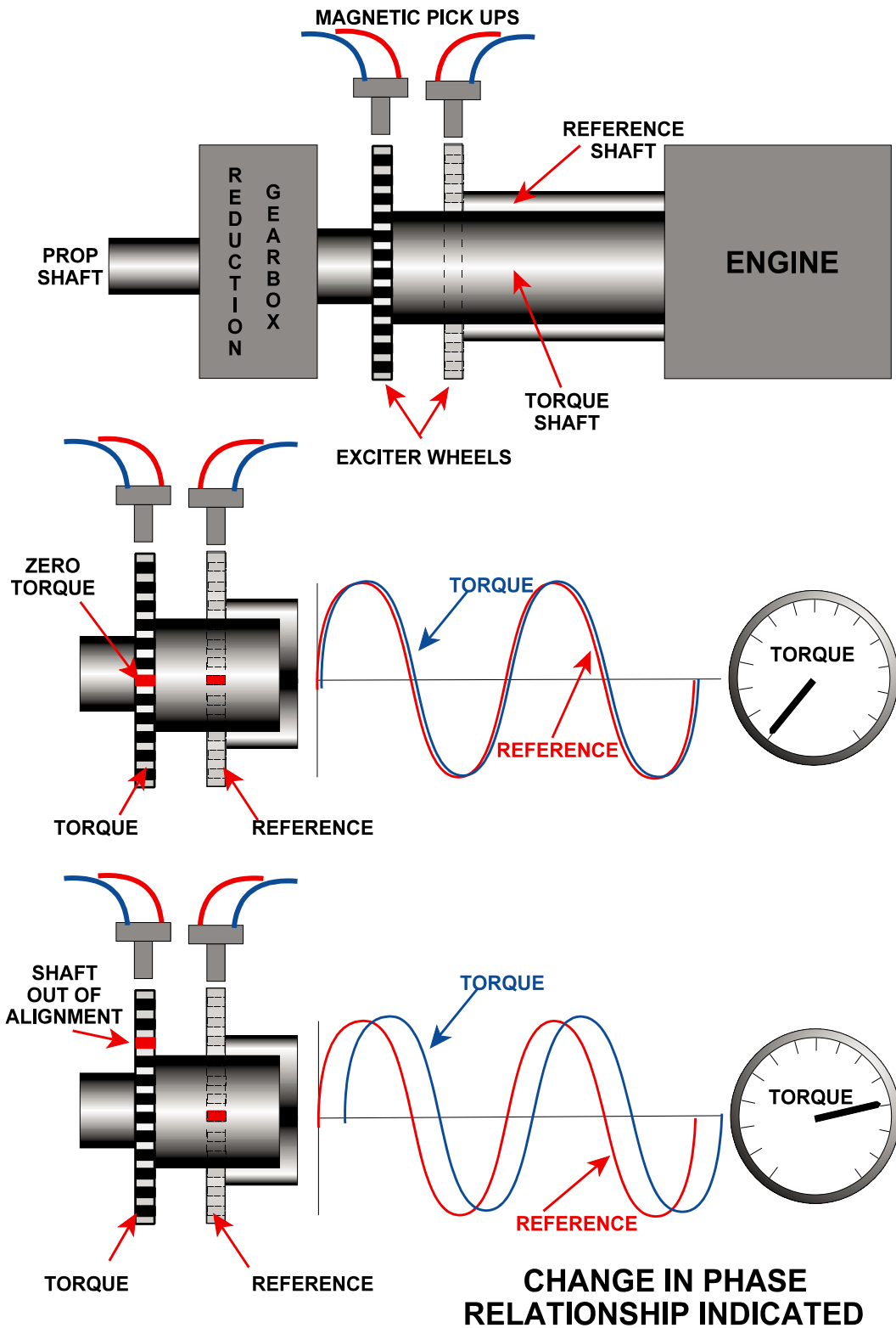
Figure 39.4 Electronic Torquemeter
