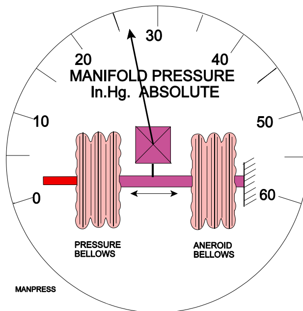
Figure 39.17 Manifold Absolute Pressure Gauge.
