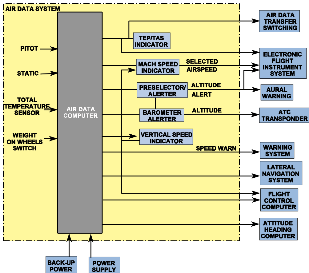
Figure 19.3 Conventional System
