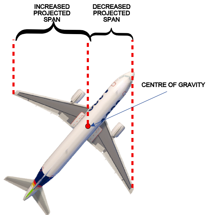
Figure 30.2 Change in Effect Aspect Ratio with Yaw
