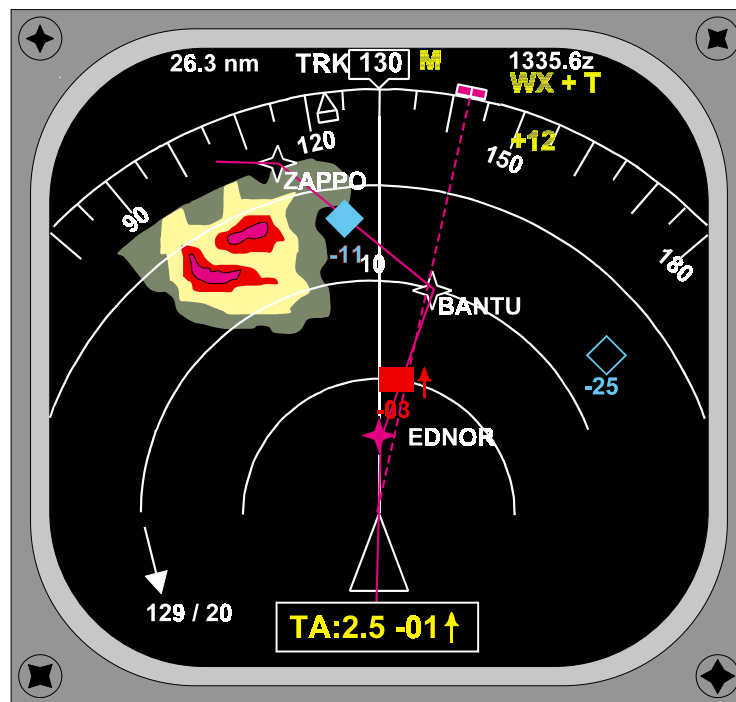
Figure 36.7a Navigation Display in MAP Mode Showing TCAS
